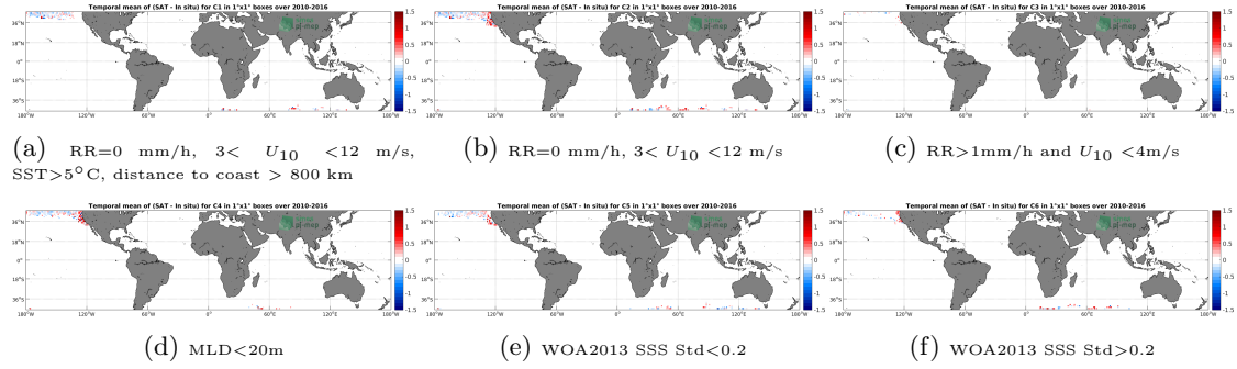
Figure 12: Temporal mean gridded over spatial boxes of size 1^\circ \times 1^\circ of \Delta SSS (SMOS-L3-ICDC-V3-MONTHLY-0.5DEG - Sea mammals) for 6 different subdatasets corresponding to: RR=0 mm/h, 3 < U_{10} < 12 m/s, SST > 5^\circ C , distance to coast > 800 km (a), RR=0 mm/h, 3 < U_{10} < 12 m/s (b), RR > 1 mm/h and U_{10} < 4 m/s (c), MLD < 20 m (d), WOA2013 SSS Std < 0.2 (e), WOA2013 SSS Std > 0.2 (f).
