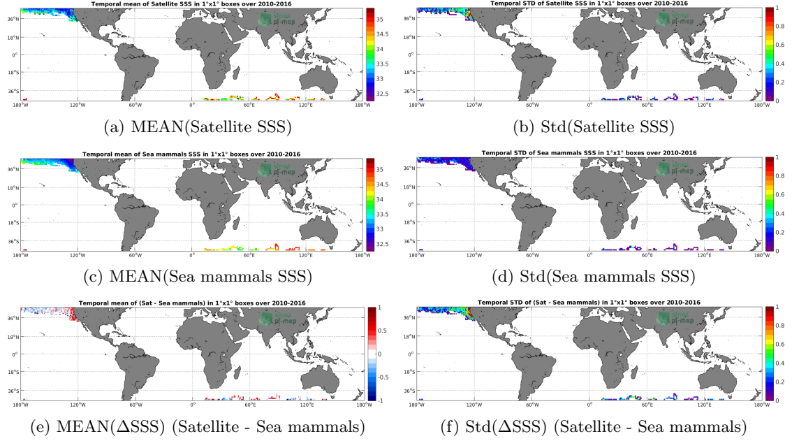
Figure 6: Temporal mean (left) and Std (right) of SSS from SMOS-L3-ICDC-V3-MONTHLY-0.5DEG (top), Sea mammals (middle), and of \Delta SSS (Satellite - Sea mammals). Only match-up pairs are used to generate these maps.
