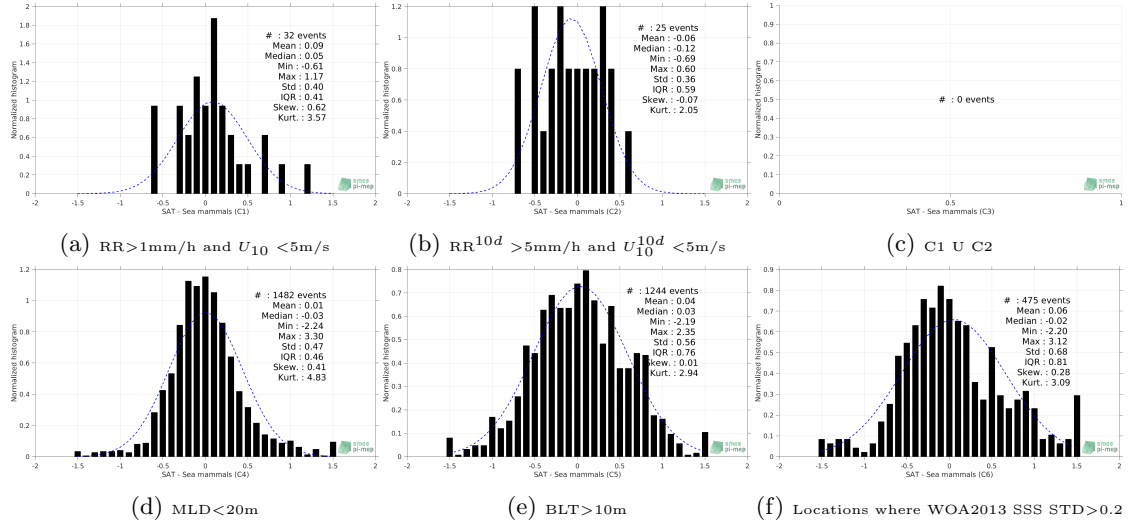
Figure 13: Normalized histogram of \Delta\text{SSS} (SMOS-L3-ICDC-V3-MONTHLY-0.5DEG - Sea mammals) for 6 different subdatasets corresponding to: \text{RR}>1\text{mm/h} and U_{10}<5\text{m/s} (a), \text{RR}^{10d}>5\text{mm/h} and U_{10}^{10d}<5\text{m/s} (b), C1 U C2 (c), \text{MLD}<20\text{m} (d), \text{BLT}>10\text{m} (e), Locations where WOA2013 SSS STD >0.2 (f).
