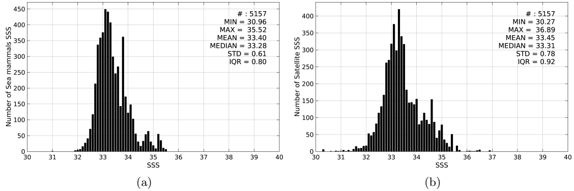
Figure 2: Histograms of SSS from Sea mammals (a) and SMOS-L3-ICDC-V3-MONTHLY-0.5DEG (b) considering all match-up pairs per bins of 0.1 over the Mid-Low Latitudes 45N-45S Pi-MEP region and for the full satellite product period.
