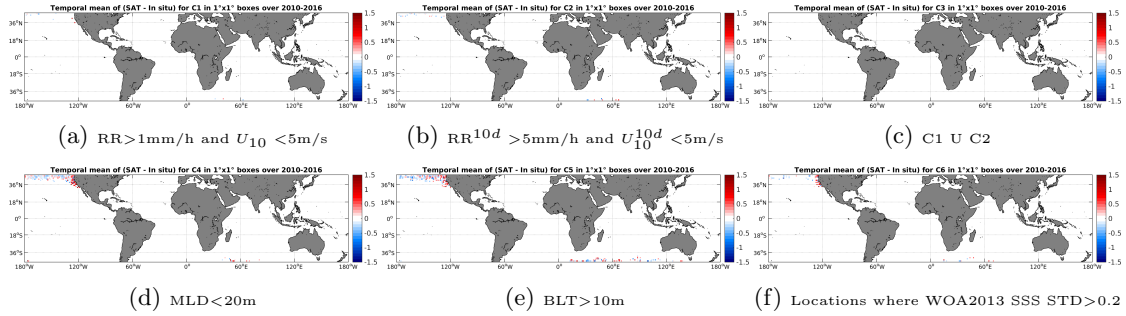
Figure 12: Temporal mean gridded over spatial boxes of size 1^\circ \times 1^\circ of \Delta SSS (SMOS-L3-ICDC-V3-MONTHLY-0.5DEG - Sea mammals) for 6 different subdatasets corresponding to: RR > 1\text{mm/h} and U_{10} < 5\text{m/s} (a), RR^{10d} > 5\text{mm/h} and U_{10}^{10d} < 5\text{m/s} (b), C1 U C2 (c), MLD < 20\text{m} (d), BLT > 10\text{m} (e), Locations where WOA2013 SSS STD > 0.2 (f).
