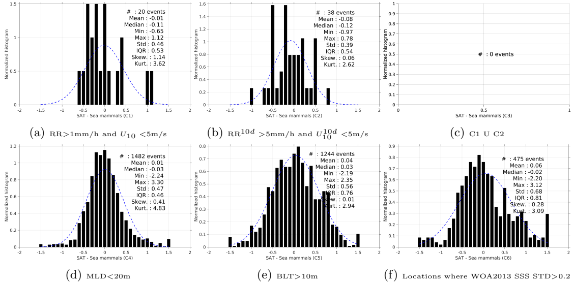
Figure 13: Normalized histogram of \Delta SSS (SMOS-L3-ICDC-V3-MONTHLY-0.5DEG - Sea mammals) for 6 different subdatasets corresponding to: RR > 1\text{mm/h} and U_{10} < 5\text{m/s} (a), RR^{10d} > 5\text{mm/h} and U_{10}^{10d} < 5\text{m/s} (b), C1 U C2 (c), MLD < 20\text{m} (d), BLT > 10\text{m} (e), Locations where WOA2013 SSS STD > 0.2 (f).
