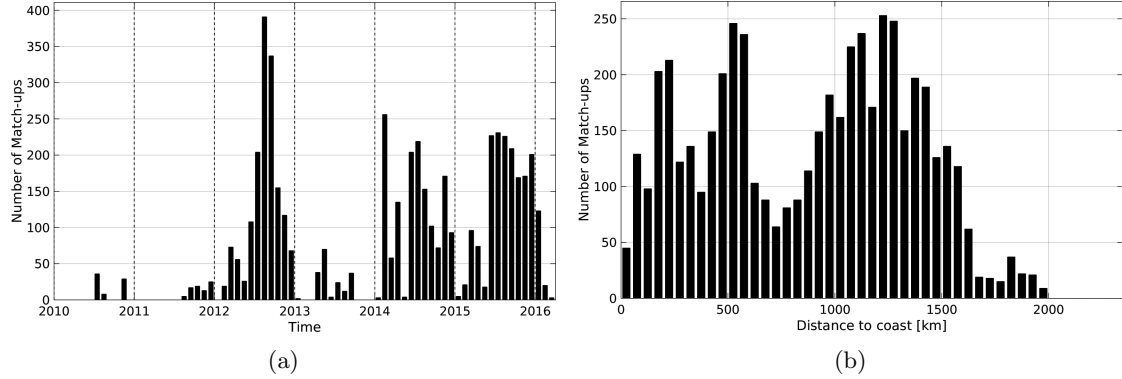
Figure 1: Number of match-ups between Sea mammals and SMOS-L3-ICDC-V3-MONTHLY-0.5DEG SSS as a function of time (a) and as function of the distance to coast (b) over the Mid-Low Latitudes 45N-45S Pi-MEP region and for the full satellite product period.
