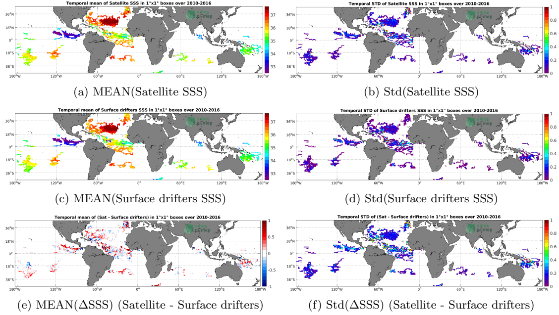
Figure 5: Temporal mean (left) and Std (right) of SSS from SMOS SSS L3 v3 Monthly (ICDC) (top), Surface drifters (middle), and of \Delta SSS (Satellite - Surface drifters). Only match-up pairs are used to generate these maps.
