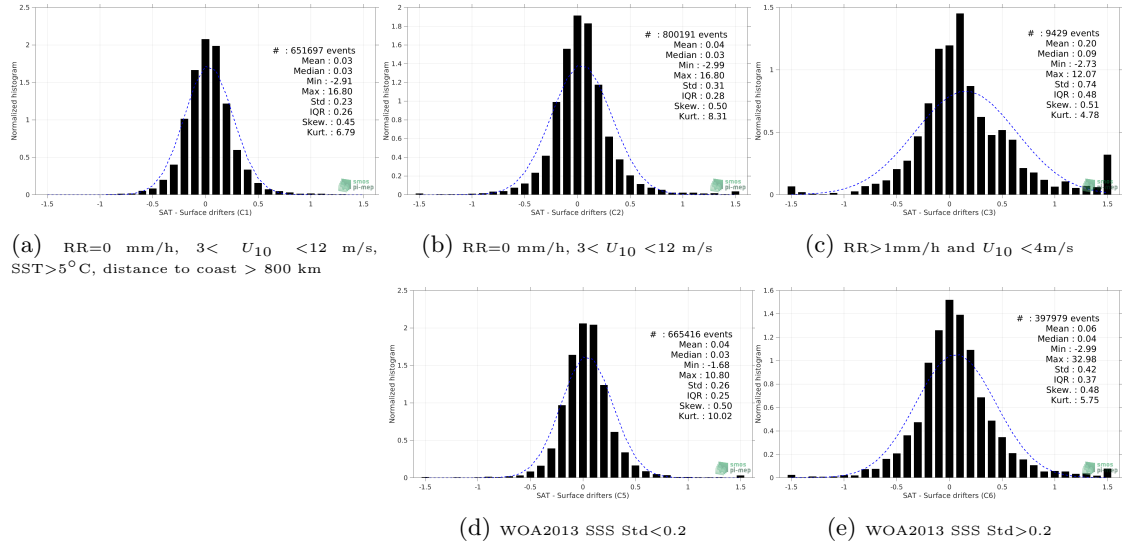
Figure 12: Normalized histogram of \Delta SSS (SMOS SSS L3 v3 Monthly (ICDC) - Surface drifters) for 5 different subdatasets corresponding to: RR=0 mm/h, 3 < U_{10} < 12 m/s, SST > 5^\circ C , distance to coast > 800 km (a), RR=0 mm/h, 3 < U_{10} < 12 m/s (b), RR > 1 mm/h and U_{10} < 4 m/s (c), WOA2013 SSS Std < 0.2 (d), WOA2013 SSS Std > 0.2 (e).
