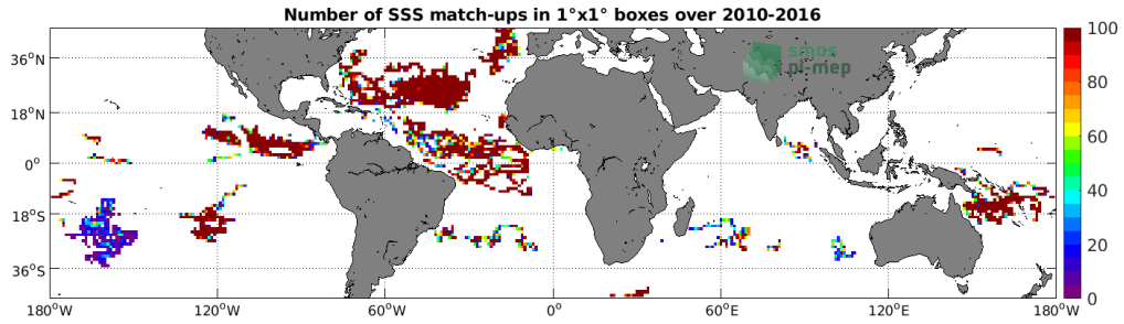
Figure 3: Number of SSS match-ups between Surface drifters SSS and the SMOS SSS L3 v3 Monthly (ICDC) SSS product for the Mid-Low Latitudes 45N-45S Pi-MEP region over 1^\circ \times 1^\circ boxes and for the full satellite product period.
