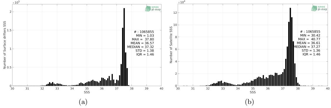
Figure 2: Histograms of SSS from Surface drifters (a) and SMOS SSS L3 v3 Monthly (ICDC) (b) considering all match-up pairs per bins of 0.1 over the Mid-Low Latitudes 45N-45S Pi-MEP region and for the full satellite product period.
