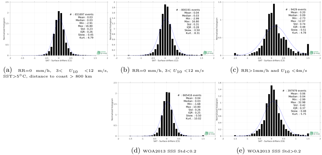
Figure 12: Normalized histogram of \Delta SSS (SMOS SSS L3 v3 Monthly (ICDC) - Surface drifters) for 5 different subdatasets corresponding to: RR=0 mm/h, 3 < U_{10} < 12 m/s, SST > 5^\circ C , distance to coast > 800 km (a), RR=0 mm/h, 3 < U_{10} < 12 m/s (b), RR > 1 mm/h and U_{10} < 4 m/s (c), WOA2013 SSS Std < 0.2 (d), WOA2013 SSS Std > 0.2 (e).
