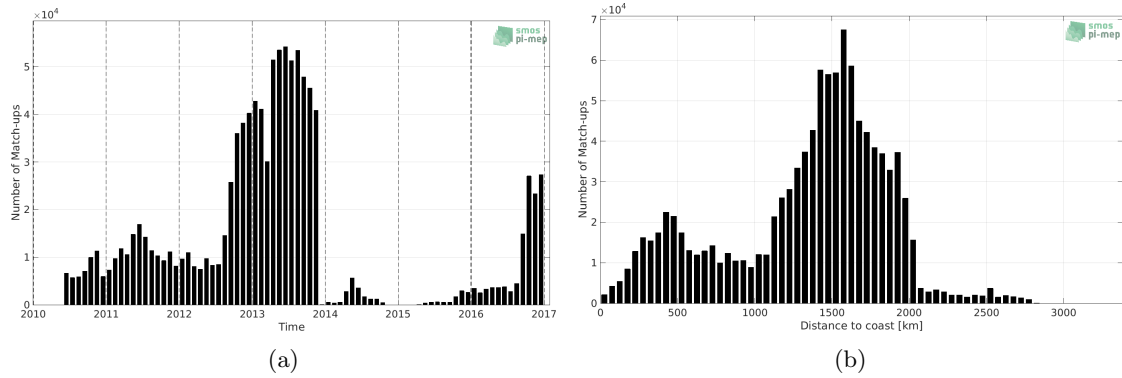
Figure 1: Number of match-ups between Surface drifters and SMOS SSS L3 v3 Monthly (ICDC) SSS as a function of time (a) and as function of the distance to coast (b) over the Mid-Low Latitudes 45N-45S Pi-MEP region and for the full satellite product period.
