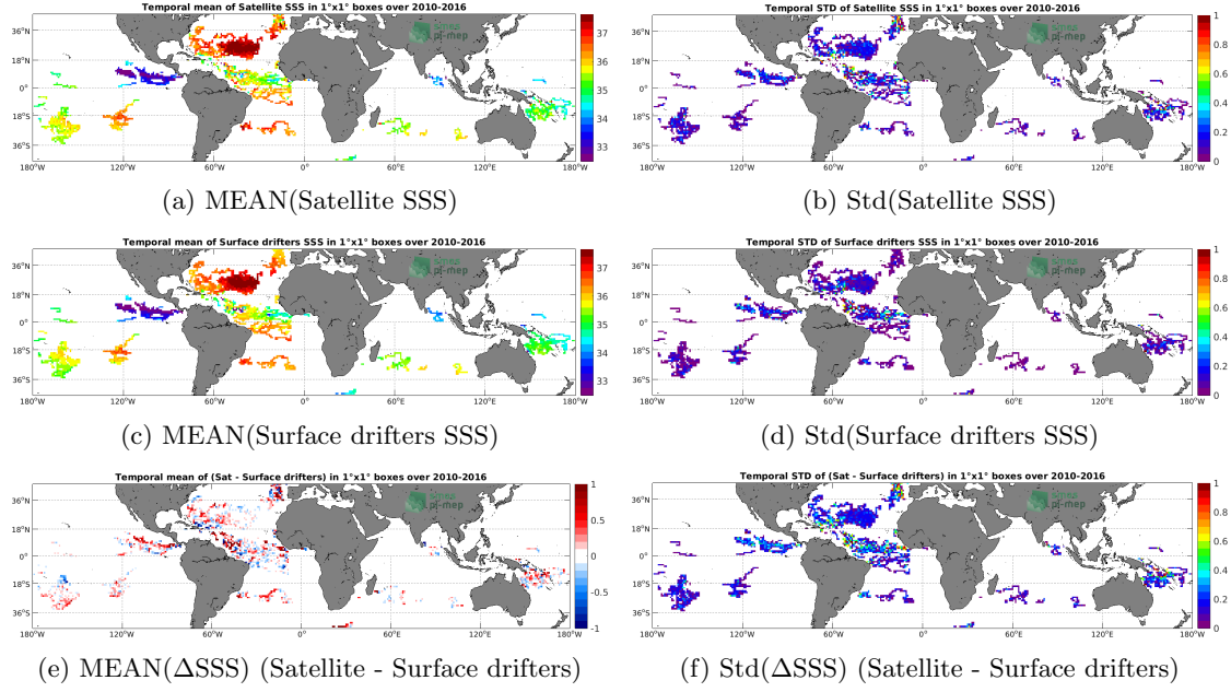
Figure 5: Temporal mean (left) and Std (right) of SSS from SMOS SSS L3 v3 Monthly (ICDC) (top), Surface drifters (middle), and of \Delta SSS (Satellite - Surface drifters). Only match-up pairs are used to generate these maps.
