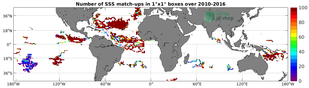
Figure 3: Number of SSS match-ups between Surface drifters SSS and the SMOS SSS L3 v3 Monthly (ICDC) SSS product for the Mid-Low Latitudes 45N-45S Pi-MEP region over 1°x1° boxes and for the full satellite product period.
