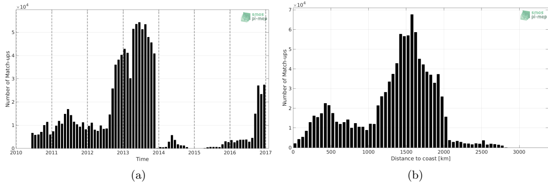
Figure 1: Number of match-ups between Surface drifters and SMOS-L3-ICDC-V3-MONTHLY-0.5DEG SSS as a function of time (a) and as function of the distance to coast (b) over the Mid-Low Latitudes 45N-45S Pi-MEP region and for the full satellite product period.
