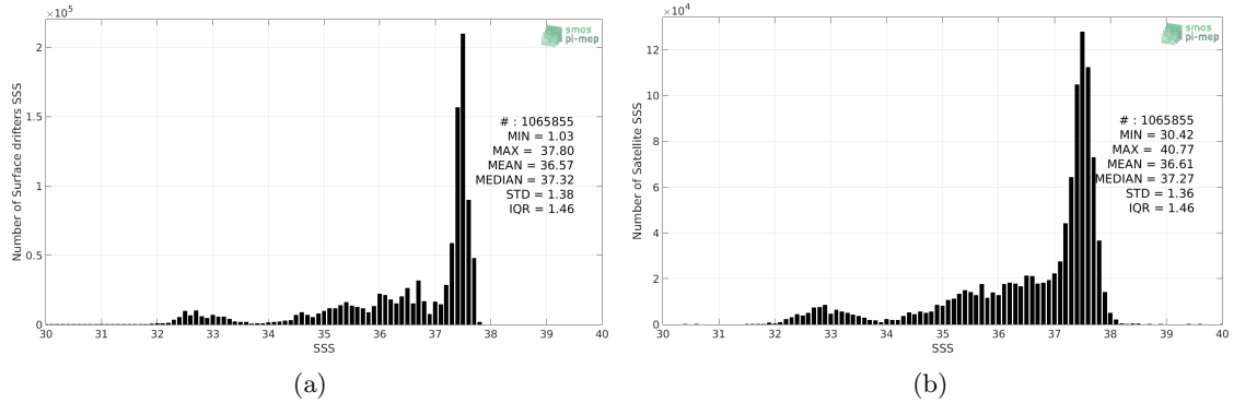
Figure 2: Histograms of SSS from Surface drifters (a) and SMOS-L3-ICDC-V3-MONTHLY-0.5DEG (b) considering all match-up pairs per bins of 0.1 over the Mid-Low Latitudes 45N-45S Pi-MEP region and for the full satellite product period.
