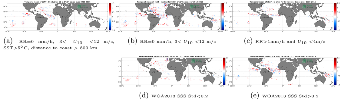
Figure 11: Temporal mean gridded over spatial boxes of size 1^\circ \times 1^\circ of \Delta SSS (SMOS-L3-ICDC-V3-MONTHLY-0.5DEG - Surface drifters) for 5 different subdatasets corresponding to: RR=0 mm/h, 3 < U_{10} < 12 m/s, SST > 5^\circ\text{C} , distance to coast > 800 km (a), RR=0 mm/h, 3 < U_{10} < 12 m/s (b), RR > 1 mm/h and U_{10} < 4 m/s (c), WOA2013 SSS Std < 0.2 (d), WOA2013 SSS Std > 0.2 (e).
