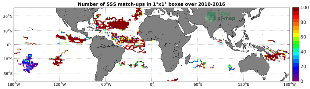
Figure 3: Number of SSS match-ups between Surface drifters SSS and the SMOS-L3-ICDC-V3-MONTHLY-0.5DEG SSS product for the Mid-Low Latitudes 45N-45S Pi-MEP region over 1°x1° boxes and for the full satellite product period.
