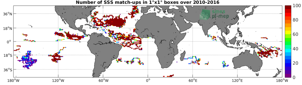
Figure 3: Number of SSS match-ups between Surface drifters SSS and the SMOS-L3-ICDC-V3-MONTHLY-0.5DEG SSS product for the Mid-Low Latitudes 45N-45S Pi-MEP region over 1^\circ \times 1^\circ boxes and for the full satellite product period.
