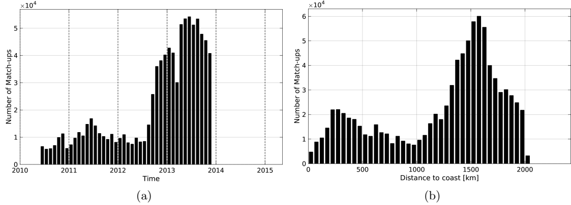
Figure 1: Number of match-ups between Surface drifters and SMOS-L3-ICDC-V3-MONTHLY-0.5DEG SSS as a function of time (a) and as function of the distance to coast (b) over the Mid-Low Latitudes 45N-45S Pi-MEP region and for the full satellite product period.
