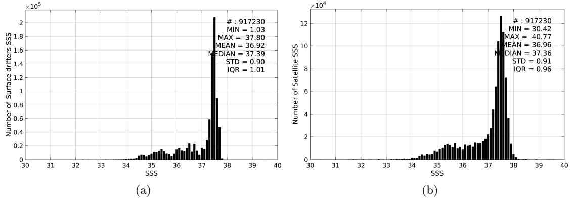
Figure 2: Histograms of SSS from Surface drifters (a) and SMOS-L3-ICDC-V3-MONTHLY-0.5DEG (b) considering all match-up pairs per bins of 0.1 over the Mid-Low Latitudes 45N-45S Pi-MEP region and for the full satellite product period.
