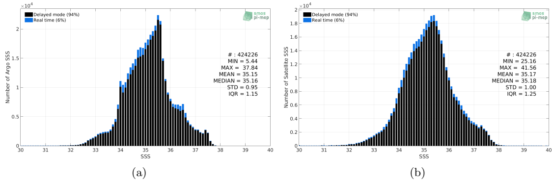
Figure 2: Histograms of SSS from Argo (a) and SMOS SSS L3 v3 Monthly (ICDC) (b) considering all match-up pairs per bins of 0.1 over the Mid-Low Latitudes 45N-45S Pi-MEP region and for the full satellite product period.
