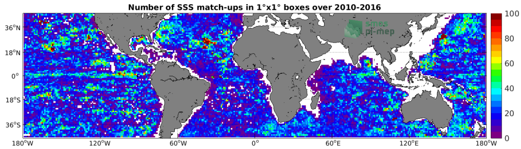
Figure 4: Number of SSS match-ups between Argo SSS and the SMOS SSS L3 v3 Monthly (ICDC) SSS product for the Mid-Low Latitudes 45N-45S Pi-MEP region over 1°x1° boxes and for the full satellite product period.
