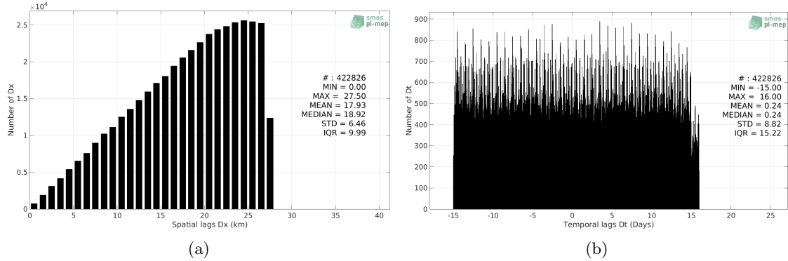
Figure 5: Histograms of the spatial (a) and temporal (b) lags between the time of the Argo measurements and the date of the corresponding SMOS SSS L3 v3 Monthly (ICDC) SSS product.
