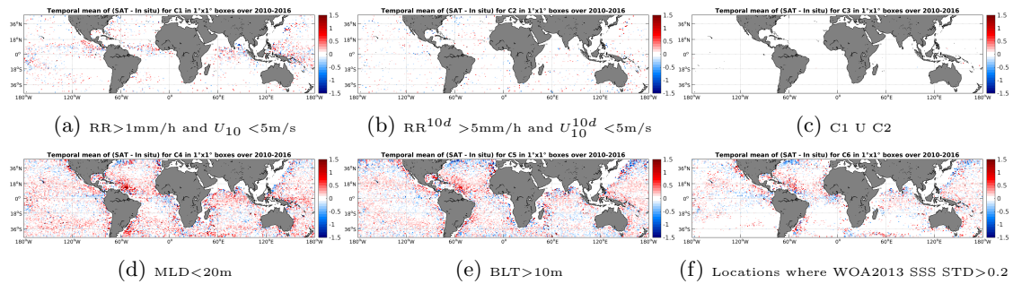
Figure 12: Temporal mean gridded over spatial boxes of size 1^\circ \times 1^\circ of \Delta SSS (SMOS-L3-ICDC-V3-MONTHLY-0.5DEG - Argo) for 6 different subdatasets corresponding to: RR>1mm/h and U_{10} < 5\text{m/s} (a), RR^{10d} > 5\text{mm/h} and U_{10}^{10d} < 5\text{m/s} (b), C1 U C2 (c), MLD<20m (d), BLT>10m (e), Locations where WOA2013 SSS STD>0.2 (f).
