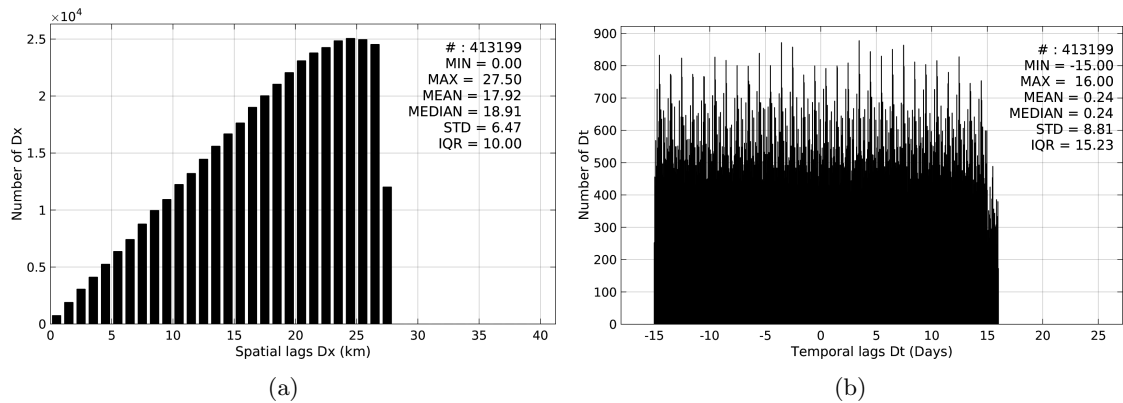
Figure 5: Histograms of the spatial (a) and temporal (b) lags between the time of the Argo measurements and the date of the corresponding SMOS-L3-ICDC-V3-MONTHLY-0.5DEG SSS product.
