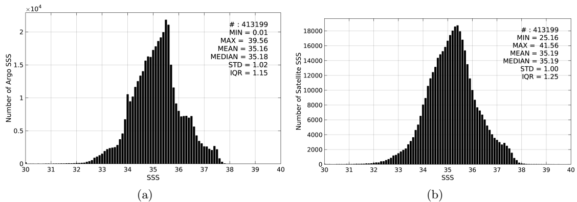
Figure 2: Histograms of SSS from Argo (a) and SMOS-L3-ICDC-V3-MONTHLY-0.5DEG (b) considering all match-up pairs per bins of 0.1 over the Mid-Low Latitudes 45N-45S Pi-MEP region and for the full satellite product period.
