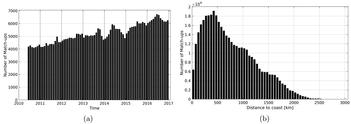
Figure 1: Number of match-ups between Argo and SMOS-L3-ICDC-V3-MONTHLY-0.5DEG SSS as a function of time (a) and as function of the distance to coast (b) over the Mid-Low Latitudes 45N-45S Pi-MEP region and for the full satellite product period.
