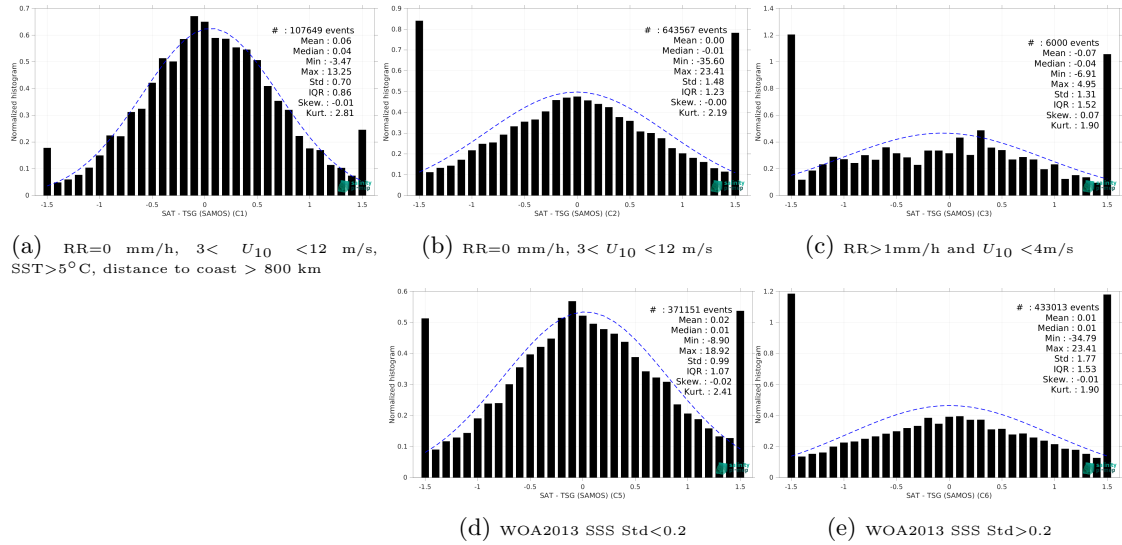
Figure 15: Normalized histogram of \Delta\text{SSS} (SMOS SSS L2Q v331 - With FLAG (CMEMS-CATDS-CPDC) - TSG (SAMOS)) for 5 different subdatasets corresponding to: RR=0 mm/h, 3 < U_{10} < 12 m/s, SST > 5^\circ\text{C} , distance to coast > 800 km (a), RR=0 mm/h, 3 < U_{10} < 12 m/s (b), RR > 1 mm/h and U_{10} < 4 m/s (c), WOA2013 SSS Std < 0.2 (d), WOA2013 SSS Std > 0.2 (e).
