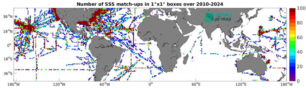
Figure 5: Number of SSS match-ups between TSG (SAMOS) SSS and the SMOS SSS L2Q v331 - With FLAG (CMEMS-CATDS-CPDC) SSS product for the Mid-Low Latitudes 45N-45S Pi-MEP region over 1^\circ \times 1^\circ boxes and for the full satellite product period.
