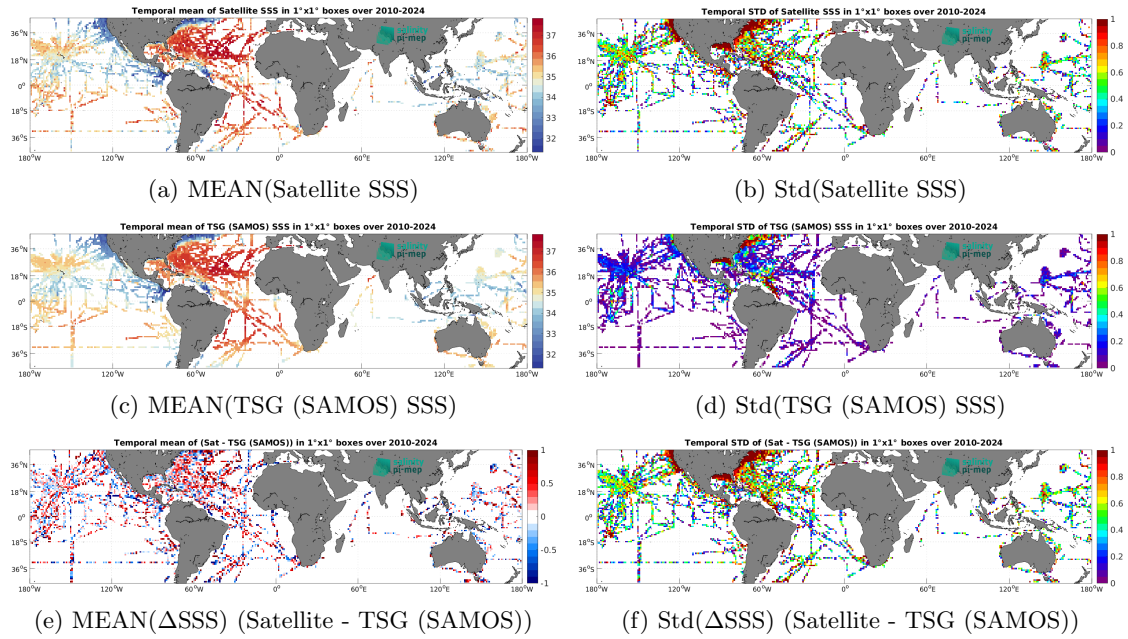
Figure 7: Temporal mean (left) and Std (right) of SSS from SMOS SSS L2Q v331 - With FLAG (CMEMS-CATDS-CPDC) (top), TSG (SAMOS) (middle), and of \Delta SSS (Satellite - TSG (SAMOS)). Only match-up pairs are used to generate these maps.
