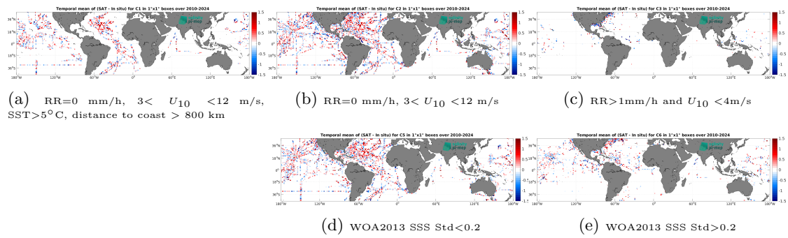
Figure 14: Temporal mean gridded over spatial boxes of size 1^\circ \times 1^\circ of \Delta\text{SSS} (SMOS SSS L2Q v331 - With FLAG (CMEMS-CATDS-CPDC) - TSG (SAMOS)) for 5 different subdatasets corresponding to: RR=0 mm/h, 3 < U_{10} < 12 m/s, SST > 5°C, distance to coast > 800 km (a), RR=0 mm/h, 3 < U_{10} < 12 m/s (b), RR > 1mm/h and U_{10} < 4 m/s (c), WOA2013 SSS Std < 0.2 (d), WOA2013 SSS Std > 0.2 (e).
