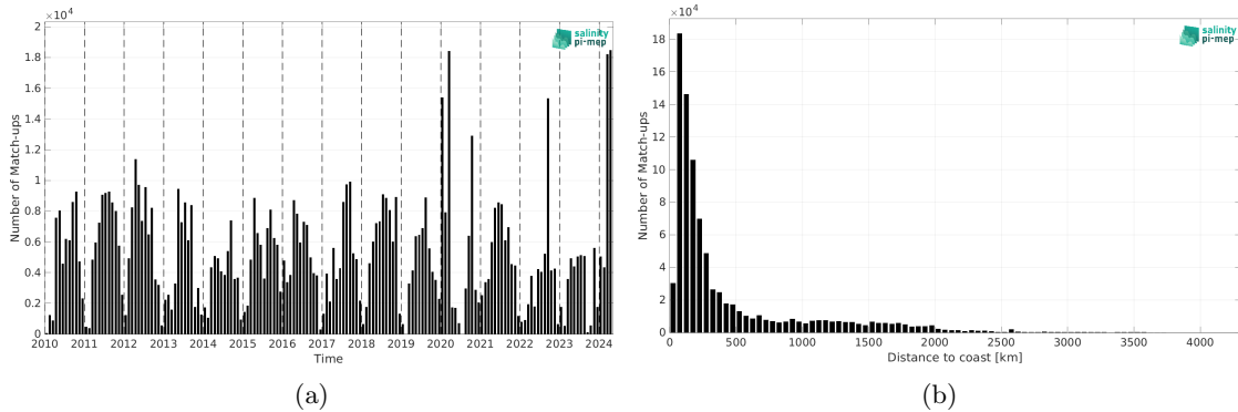
Figure 2: Number of match-ups between TSG (SAMOS) and SMOS SSS L2Q v331 - With FLAG (CMEMS-CATDS-CPDC) SSS as a function of time (a) and as function of the distance to coast (b) over the Mid-Low Latitudes 45N-45S Pi-MEP region and for the full satellite product period.
