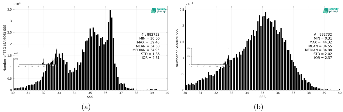
Figure 3: Histograms of SSS from TSG (SAMOS) (a) and SMOS SSS L2Q v331 - With FLAG (CMEMS-CATDS-CPDC) (b) considering all match-up pairs per bins of 0.1 over the Mid-Low Latitudes 45N-45S Pi-MEP region and for the full satellite product period.
