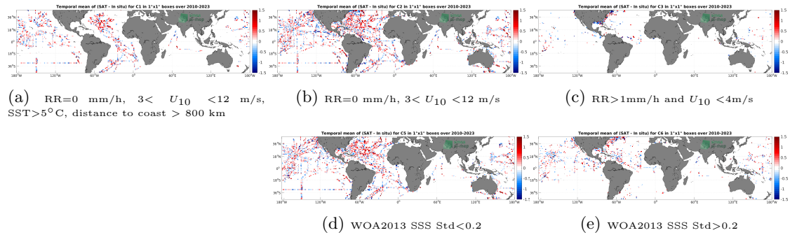
Figure 12: Temporal mean gridded over spatial boxes of size 1^\circ \times 1^\circ of \Delta SSS (SMOS SSS L2Q v331 - With FLAG (CMEMS-CATDS-CPDC) - TSG (SAMOS)) for 5 different subdatasets corresponding to:RR=0 mm/h, 3 < U_{10} < 12 m/s, SST >5^\circ\text{C} , distance to coast > 800 km (a), RR=0 mm/h, 3 < U_{10} < 12 m/s (b), RR >1 mm/h and U_{10} < 4 m/s (c), WOA2013 SSS Std <0.2 (d), WOA2013 SSS Std >0.2 (e).
