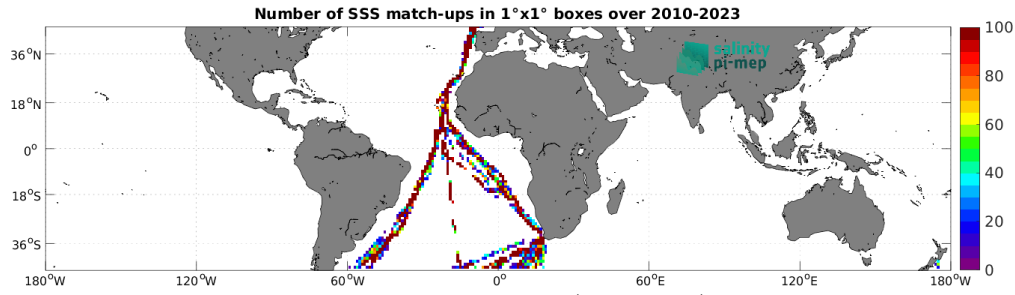
Figure 5: Number of SSS match-ups between TSG (Polarstern) SSS and the SMOS SSS L2Q v331 - With FLAG (CMEMS-CATDS-CPDC) SSS product for the Mid-Low Latitudes 45N-45S Pi-MEP region over 1^\circ \times 1^\circ boxes and for the full satellite product period.
