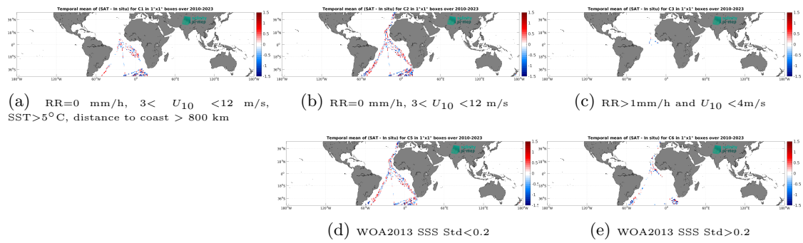
Figure 14: Temporal mean gridded over spatial boxes of size 1^\circ \times 1^\circ of \Delta SSS (SMOS SSS L2Q v331 - With FLAG (CMEMS-CATDS-CPDC) - TSG (Polarstern)) for 5 different subdatasets corresponding to:RR=0 mm/h, 3 < U_{10} < 12 m/s, SST>5°C, distance to coast > 800 km (a), RR=0 mm/h, 3 < U_{10} < 12 m/s (b), RR>1mm/h and U_{10} < 4 m/s (c), WOA2013 SSS Std<0.2 (d), WOA2013 SSS Std>0.2 (e).
