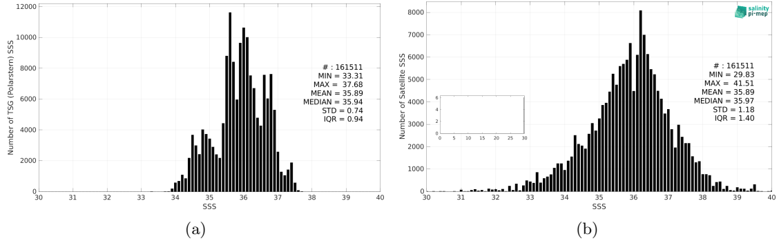
Figure 3: Histograms of SSS from TSG (Polarstern) (a) and SMOS SSS L2Q v331 - With FLAG (CMEMS-CATDS-CPDC) (b) considering all match-up pairs per bins of 0.1 over the Mid-Low Latitudes 45N-45S Pi-MEP region and for the full satellite product period.
