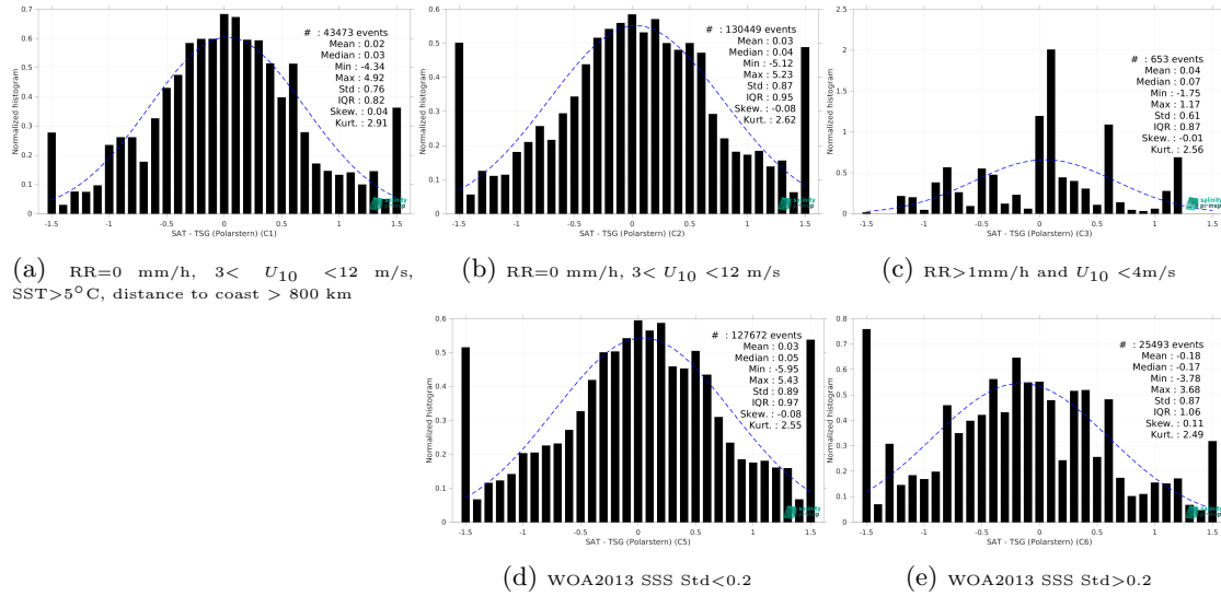
Figure 15: Normalized histogram of \Delta SSS (SMOS SSS L2Q v331 - With FLAG (CMEMS-CATDS-CPDC) - TSG (Polarstern)) for 5 different subdatasets corresponding to: RR=0 mm/h, 3 < U_{10} < 12 m/s, SST>5°C, distance to coast > 800 km (a), RR=0 mm/h, 3 < U_{10} < 12 m/s (b), RR>1mm/h and U_{10} < 4 m/s (c), WOA2013 SSS Std<0.2 (d), WOA2013 SSS Std>0.2 (e).
