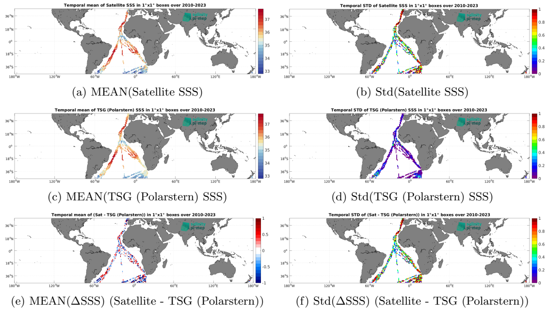
Figure 7: Temporal mean (left) and Std (right) of SSS from SMOS SSS L2Q v331 - With FLAG (CMEMS-CATDS-CPDC) (top), TSG (Polarstern) (middle), and of \Delta SSS (Satellite - TSG (Polarstern)). Only match-up pairs are used to generate these maps.
