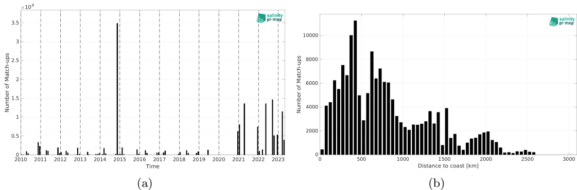
Figure 2: Number of match-ups between TSG (Polarstern) and SMOS SSS L2Q v331 - With FLAG (CMEMS-CATDS-CPDC) SSS as a function of time (a) and as function of the distance to coast (b) over the Mid-Low Latitudes 45N-45S Pi-MEP region and for the full satellite product period.
