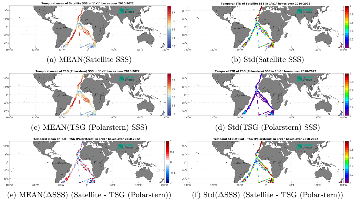
Figure 6: Temporal mean (left) and Std (right) of SSS from SMOS SSS L2Q v331 - With FLAG (CMEMS-CATDS-CPDC) (top), TSG (Polarstern) (middle), and of \Delta SSS (Satellite - TSG (Polarstern)). Only match-up pairs are used to generate these maps.
