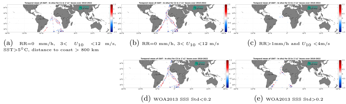
Figure 12: Temporal mean gridded over spatial boxes of size 1^\circ \times 1^\circ of \Delta SSS (SMOS SSS L2Q v331 - With FLAG (CMEMS-CATDS-CPDC) - TSG (Polarstern)) for 5 different subdatasets corresponding to:RR=0 mm/h, 3 < U_{10} < 12 m/s, SST >5^\circ C, distance to coast > 800 km (a), RR=0 mm/h, 3 < U_{10} < 12 m/s (b), RR >1 mm/h and U_{10} < 4 m/s (c), WOA2013 SSS Std <0.2 (d), WOA2013 SSS Std >0.2 (e).
