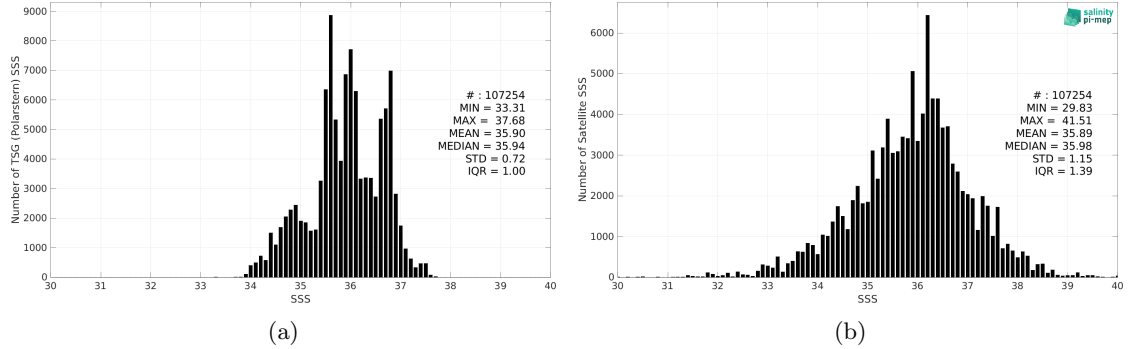
Figure 2: Histograms of SSS from TSG (Polarstern) (a) and SMOS SSS L2Q v331 - With FLAG (CMEMS-CATDS-CPDC) (b) considering all match-up pairs per bins of 0.1 over the Mid-Low Latitudes 45N-45S Pi-MEP region and for the full satellite product period.
