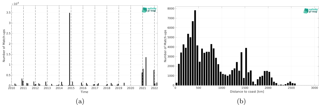
Figure 1: Number of match-ups between TSG (Polarstern) and SMOS SSS L2Q v331 - With FLAG (CMEMS-CATDS-CPDC) SSS as a function of time (a) and as function of the distance to coast (b) over the Mid-Low Latitudes 45N-45S Pi-MEP region and for the full satellite product period.
