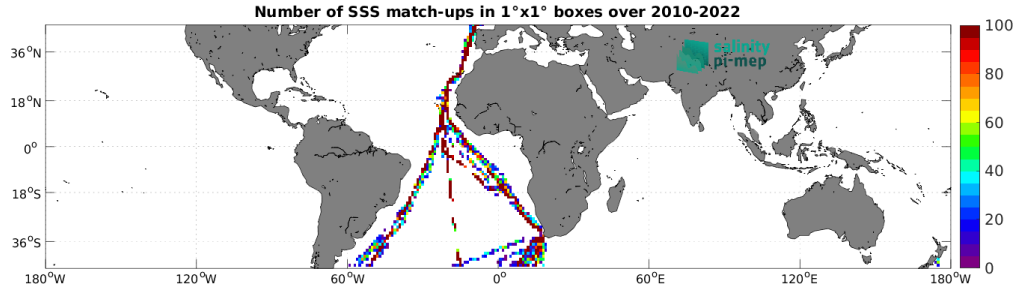
Figure 4: Number of SSS match-ups between TSG (Polarstern) SSS and the SMOS SSS L2Q v331 - With FLAG (CMEMS-CATDS-CPDC) SSS product for the Mid-Low Latitudes 45N-45S Pi-MEP region over 1^\circ \times 1^\circ boxes and for the full satellite product period.
