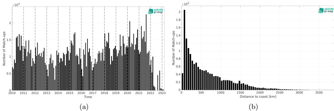
Figure 2: Number of match-ups between TSG (LEGOS-DM) and SMOS SSS L2Q v331 - With FLAG (CMEMS-CATDS-CPDC) SSS as a function of time (a) and as function of the distance to coast (b) over the Mid-Low Latitudes 45N-45S Pi-MEP region and for the full satellite product period.
