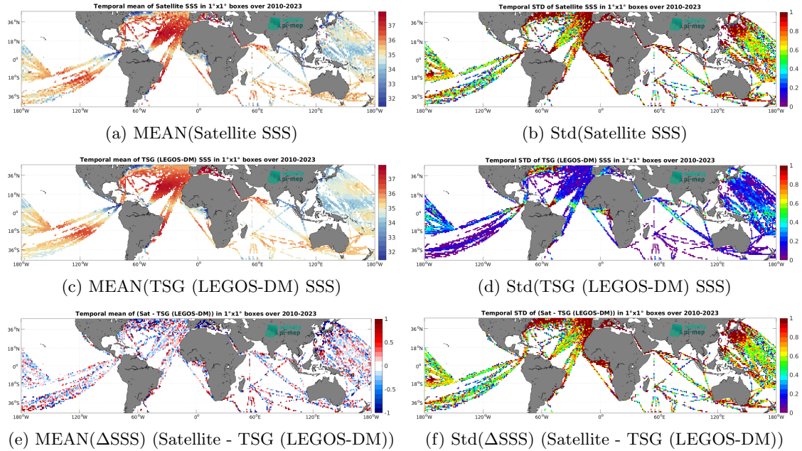
Figure 7: Temporal mean (left) and Std (right) of SSS from SMOS SSS L2Q v331 - With FLAG (CMEMS-CATDS-CPDC) (top), TSG (LEGOS-DM) (middle), and of \Delta SSS (Satellite - TSG (LEGOS-DM)). Only match-up pairs are used to generate these maps.
