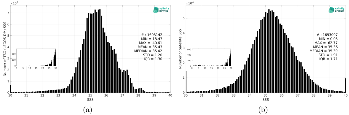
Figure 3: Histograms of SSS from TSG (LEGOS-DM) (a) and SMOS SSS L2Q v331 - With FLAG (CMEMS-CATDS-CPDC) (b) considering all match-up pairs per bins of 0.1 over the Mid-Low Latitudes 45N-45S Pi-MEP region and for the full satellite product period.
