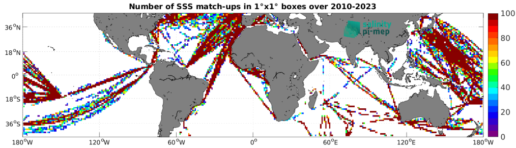
Figure 5: Number of SSS match-ups between TSG (LEGOS-DM) SSS and the SMOS SSS L2Q v331 - With FLAG (CMEMS-CATDS-CPDC) SSS product for the Mid-Low Latitudes 45N-45S Pi-MEP region over 1^\circ \times 1^\circ boxes and for the full satellite product period.
