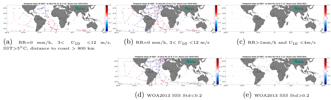
Figure 14: Temporal mean gridded over spatial boxes of size 1^\circ \times 1^\circ of \Delta\text{SSS} (SMOS SSS L2Q v331 - With FLAG (CMEMS-CATDS-CPDC) - TSG (GOSUD-Sailing-ship)) for 5 different subdatasets corresponding to: RR=0 mm/h, 3 < U_{10} < 12 m/s, SST > 5°C, distance to coast > 800 km (a), RR=0 mm/h, 3 < U_{10} < 12 m/s (b), RR > 1mm/h and U_{10} < 4 m/s (c), WOA2013 SSS Std < 0.2 (d), WOA2013 SSS Std > 0.2 (e).
