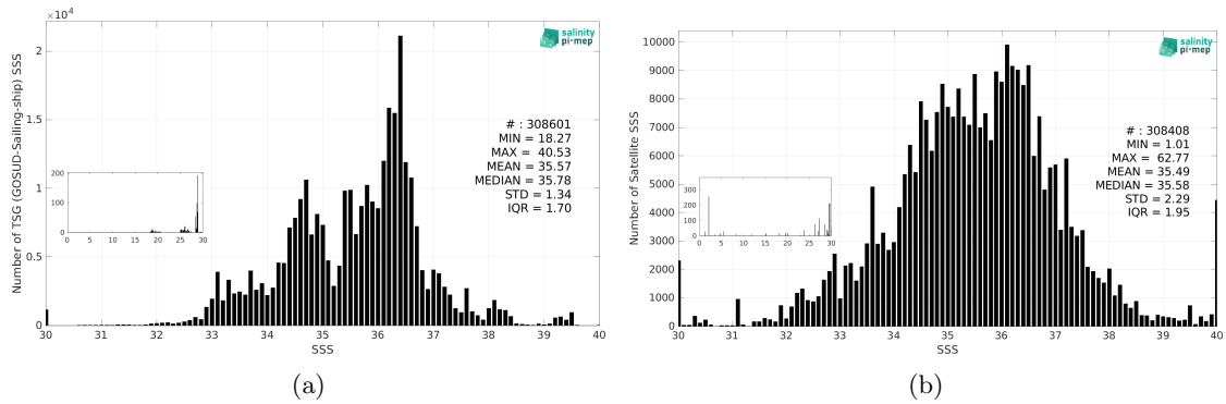
Figure 3: Histograms of SSS from TSG (GOSUD-Sailing-ship) (a) and SMOS SSS L2Q v331 - With FLAG (CMEMS-CATDS-CPDC) (b) considering all match-up pairs per bins of 0.1 over the Mid-Low Latitudes 45N-45S Pi-MEP region and for the full satellite product period.
