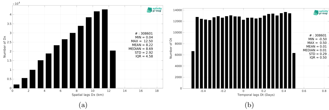
Figure 5: Histograms of the spatial (a) and temporal (b) lags between the location/time of the TSG (GOSUD-Sailing-ship) measurement and the date of the corresponding SMOS SSS L2Q v331 - With FLAG (CMEMS-CATDS-CPDC) SSS pixel.
