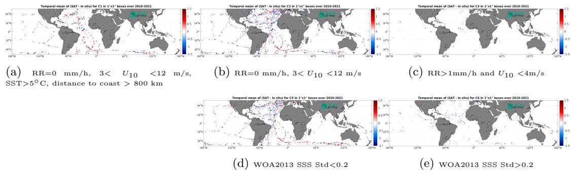
Figure 12: Temporal mean gridded over spatial boxes of size 1^\circ \times 1^\circ of \Delta\text{SSS} (SMOS SSS L2Q v331 - With FLAG (CMEMS-CATDS-CPDC) - TSG (GOSUD-Sailing-ship)) for 5 different subdatasets corresponding to:RR=0 mm/h, 3 < U_{10} < 12 m/s, SST >5^\circ\text{C} , distance to coast > 800 km (a), RR=0 mm/h, 3 < U_{10} < 12 m/s (b), RR >1 mm/h and U_{10} < 4 m/s (c), WOA2013 SSS Std <0.2 (d), WOA2013 SSS Std >0.2 (e).
