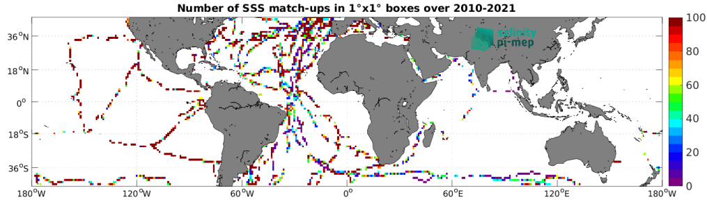
Figure 4: Number of SSS match-ups between TSG (GOSUD-Sailing-ship) SSS and the SMOS SSS L2Q v331 - With FLAG (CMEMS-CATDS-CPDC) SSS product for the Mid-Low Latitudes 45N-45S Pi-MEP region over 1^\circ \times 1^\circ boxes and for the full satellite product period.
