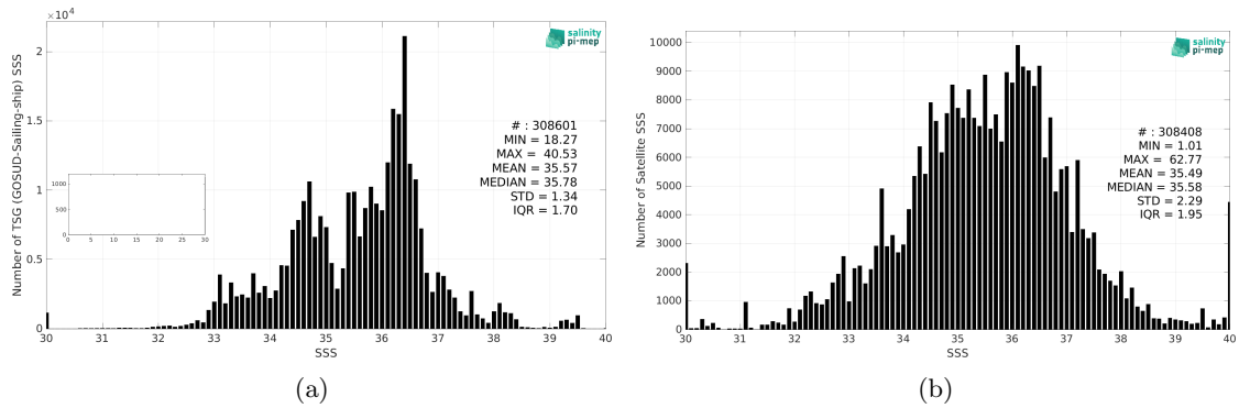
Figure 2: Histograms of SSS from TSG (GOSUD-Sailing-ship) (a) and SMOS SSS L2Q v331 - With FLAG (CMEMS-CATDS-CPDC) (b) considering all match-up pairs per bins of 0.1 over the Mid-Low Latitudes 45N-45S Pi-MEP region and for the full satellite product period.
