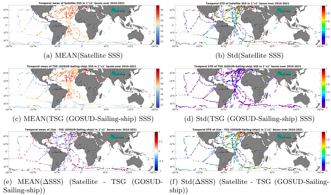
Figure 6: Temporal mean (left) and Std (right) of SSS from SMOS SSS L2Q v331 - With FLAG (CMEMS-CATDS-CPDC) (top), TSG (GOSUD-Sailing-ship) (middle), and of \Delta SSS (Satellite - TSG (GOSUD-Sailing-ship)). Only match-up pairs are used to generate these maps.
