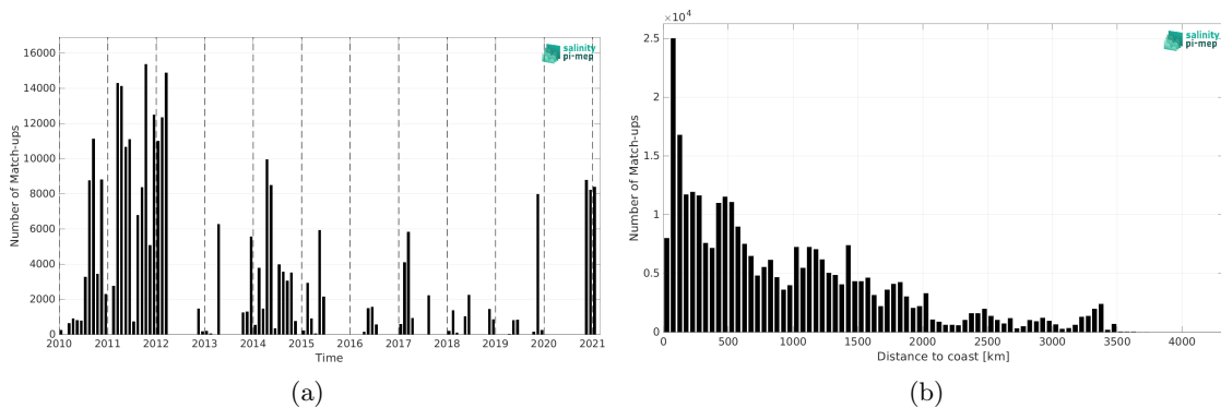
Figure 1: Number of match-ups between TSG (GOSUD-Sailing-ship) and SMOS SSS L2Q v331 - With FLAG (CMEMS-CATDS-CPDC) SSS as a function of time (a) and as function of the distance to coast (b) over the Mid-Low Latitudes 45N-45S Pi-MEP region and for the full satellite product period.
