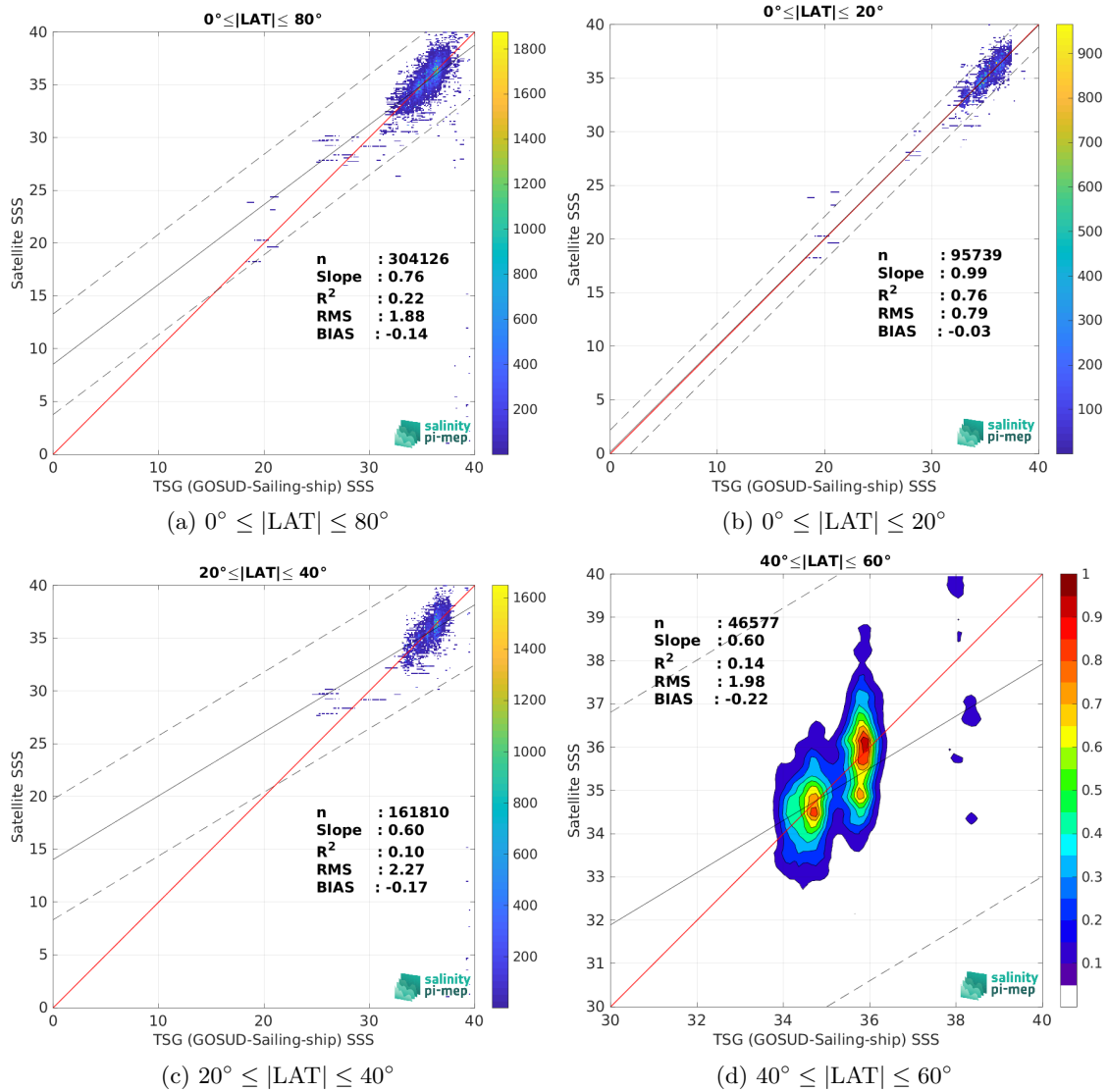
Figure 9: Contour maps of the concentration of SMOS SSS L2Q v331 - With FLAG (CMEMS-CATDS-CPDC) SSS (y-axis) versus TSG (GOSUD-Sailing-ship) SSS (x-axis) at match-up pairs for different latitude bands. For each plot, the red line shows x=y . The black thin and dashed lines indicate a linear fit through the data cloud and the \pm 95\% confidence levels, respectively. The number match-up pairs n , the slope and R^2 coefficient of the linear fit, the root mean square (RMS) and the mean bias between satellite and in situ data are indicated for each latitude band in each plots.
