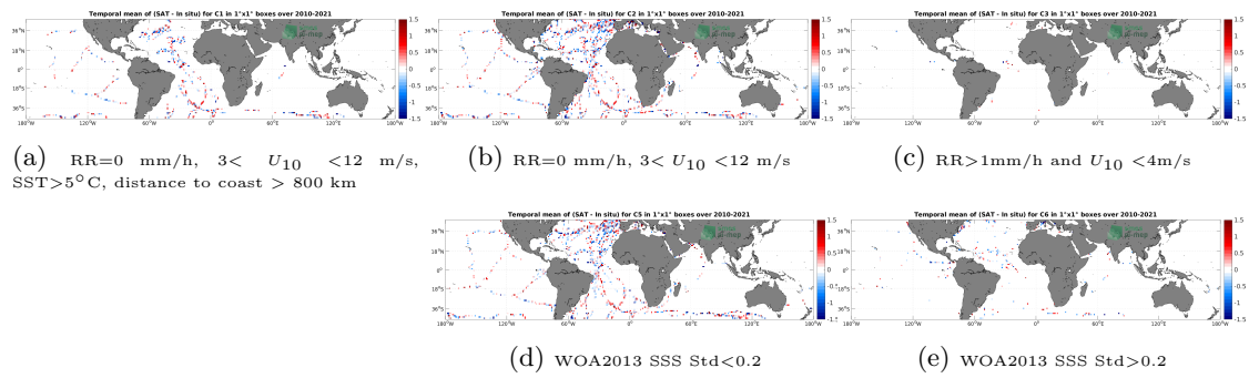
Figure 12: Temporal mean gridded over spatial boxes of size 1^\circ \times 1^\circ of \Delta SSS (SMOS SSS L2Q v331 - With FLAG (CMEMS-CATDS-CPDC) - TSG (GOSUD-Sailing-ship)) for 5 different subdatasets corresponding to:RR=0 mm/h, 3 < U_{10} < 12 m/s, SST >5^\circ C, distance to coast > 800 km (a), RR=0 mm/h, 3 < U_{10} < 12 m/s (b), RR >1 mm/h and U_{10} < 4 m/s (c), WOA2013 SSS Std <0.2 (d), WOA2013 SSS Std >0.2 (e).
