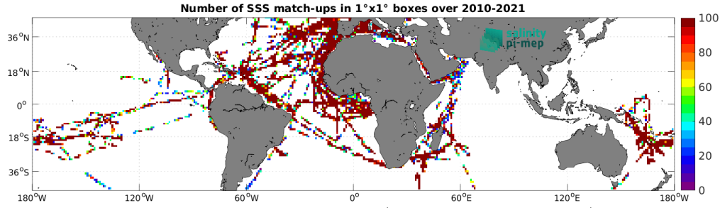
Figure 5: Number of SSS match-ups between TSG (GOSUD-Research-vessel) SSS and the SMOS SSS L2Q v331 - With FLAG (CMEMS-CATDS-CPDC) SSS product for the Mid-Low Latitudes 45N-45S Pi-MEP region over 1^\circ \times 1^\circ boxes and for the full satellite product period.
