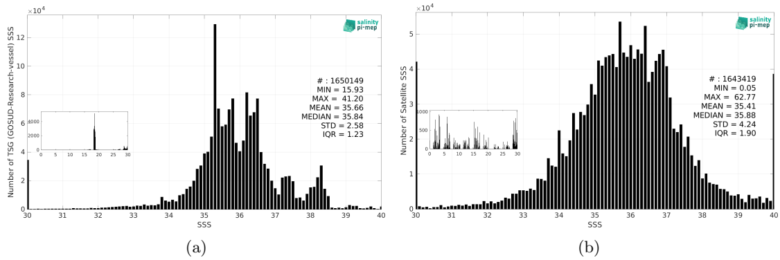
Figure 3: Histograms of SSS from TSG (GOSUD-Research-vessel) (a) and SMOS SSS L2Q v331 - With FLAG (CMEMS-CATDS-CPDC) (b) considering all match-up pairs per bins of 0.1 over the Mid-Low Latitudes 45N-45S Pi-MEP region and for the full satellite product period.
