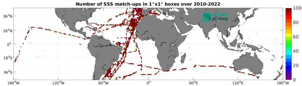
Figure 5: Number of SSS match-ups between TSG (CSIC-UTM) SSS and the SMOS SSS L2Q v331 - With FLAG (CMEMS-CATDS-CPDC) SSS product for the Mid-Low Latitudes 45N-45S Pi-MEP region over 1^\circ \times 1^\circ boxes and for the full satellite product period.
