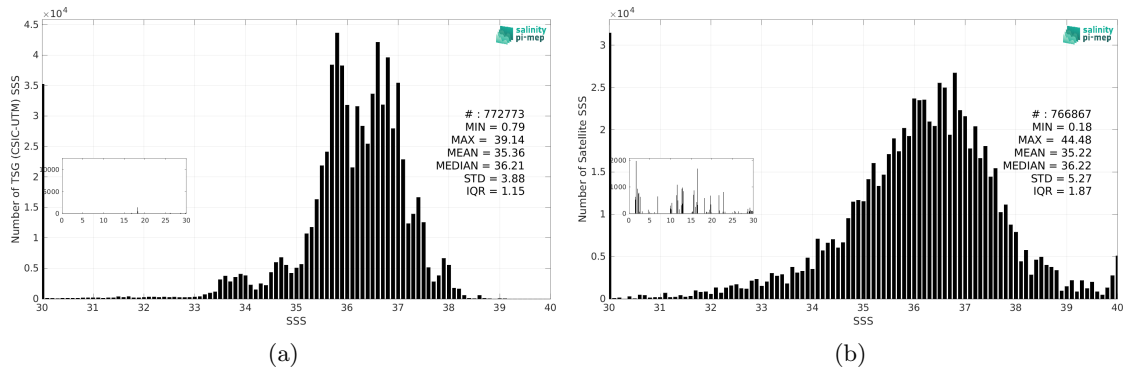
Figure 3: Histograms of SSS from TSG (CSIC-UTM) (a) and SMOS SSS L2Q v331 - With FLAG (CMEMS-CATDS-CPDC) (b) considering all match-up pairs per bins of 0.1 over the Mid-Low Latitudes 45N-45S Pi-MEP region and for the full satellite product period.
