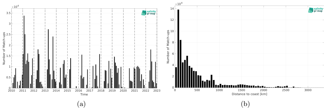
Figure 2: Number of match-ups between TSG (CSIC-UTM) and SMOS SSS L2Q v331 - With FLAG (CMEMS-CATDS-CPDC) SSS as a function of time (a) and as function of the distance to coast (b) over the Mid-Low Latitudes 45N-45S Pi-MEP region and for the full satellite product period.
