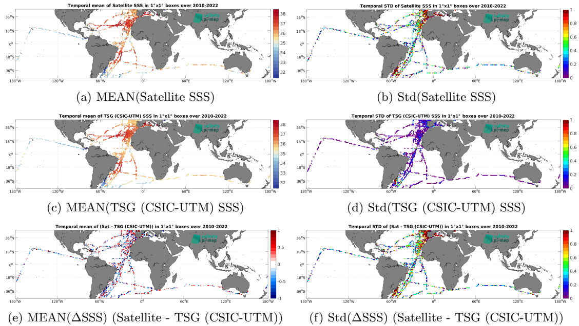
Figure 6: Temporal mean (left) and Std (right) of SSS from SMOS SSS L2Q v331 - With FLAG (CMEMS-CATDS-CPDC) (top), TSG (CSIC-UTM) (middle), and of \Delta SSS (Satellite - TSG (CSIC-UTM)). Only match-up pairs are used to generate these maps.
