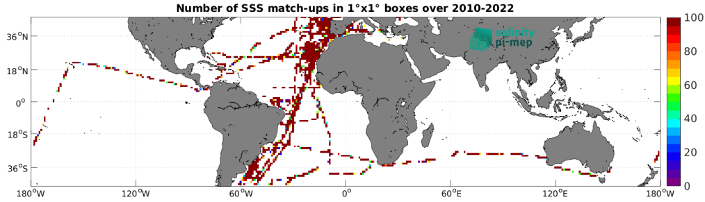
Figure 4: Number of SSS match-ups between TSG (CSIC-UTM) SSS and the SMOS SSS L2Q v331 - With FLAG (CMEMS-CATDS-CPDC) SSS product for the Mid-Low Latitudes 45N-45S Pi-MEP region over 1^\circ \times 1^\circ boxes and for the full satellite product period.
