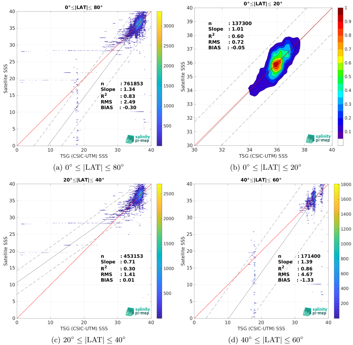
Figure 9: Contour maps of the concentration of SMOS SSS L2Q v331 - With FLAG (CMEMS-CATDS-CPDC) SSS (y-axis) versus TSG (CSIC-UTM) SSS (x-axis) at match-up pairs for different latitude bands. For each plot, the red line shows x=y . The black thin and dashed lines indicate a linear fit through the data cloud and the \pm 95\% confidence levels, respectively. The number match-up pairs n , the slope and R^2 coefficient of the linear fit, the root mean square (RMS) and the mean bias between satellite and in situ data are indicated for each latitude band in each plots.
