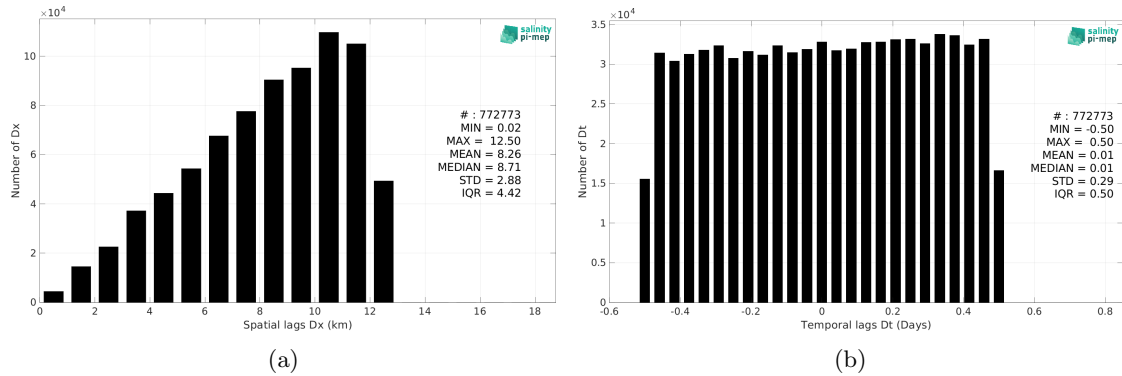
Figure 5: Histograms of the spatial (a) and temporal (b) lags between the location/time of the TSG (CSIC-UTM) measurement and the date of the corresponding SMOS SSS L2Q v331 - With FLAG (CMEMS-CATDS-CPDC) SSS pixel.
