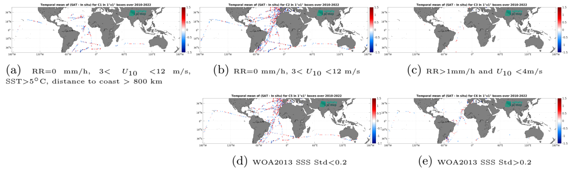
Figure 12: Temporal mean gridded over spatial boxes of size 1^\circ \times 1^\circ of \Delta SSS (SMOS SSS L2Q v331 - With FLAG (CMEMS-CATDS-CPDC) - TSG (CSIC-UTM)) for 5 different subdatasets corresponding to:RR=0 mm/h, 3 < U_{10} < 12 m/s, SST >5^\circ\text{C} , distance to coast > 800 km (a), RR=0 mm/h, 3 < U_{10} < 12 m/s (b), RR >1 mm/h and U_{10} < 4 m/s (c), WOA2013 SSS Std <0.2 (d), WOA2013 SSS Std >0.2 (e).
