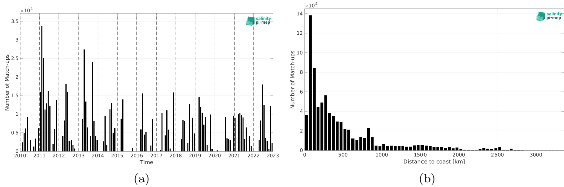
Figure 1: Number of match-ups between TSG (CSIC-UTM) and SMOS SSS L2Q v331 - With FLAG (CMEMS-CATDS-CPDC) SSS as a function of time (a) and as function of the distance to coast (b) over the Mid-Low Latitudes 45N-45S Pi-MEP region and for the full satellite product period.
