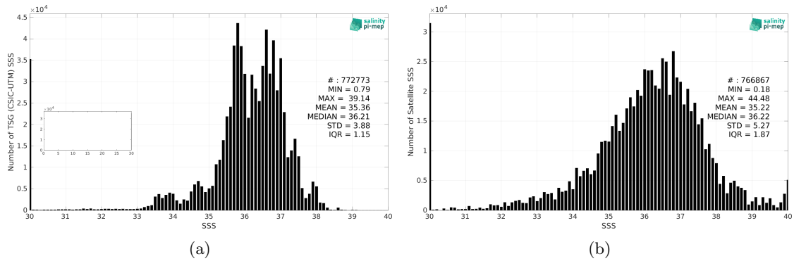
Figure 2: Histograms of SSS from TSG (CSIC-UTM) (a) and SMOS SSS L2Q v331 - With FLAG (CMEMS-CATDS-CPDC) (b) considering all match-up pairs per bins of 0.1 over the Mid-Low Latitudes 45N-45S Pi-MEP region and for the full satellite product period.
