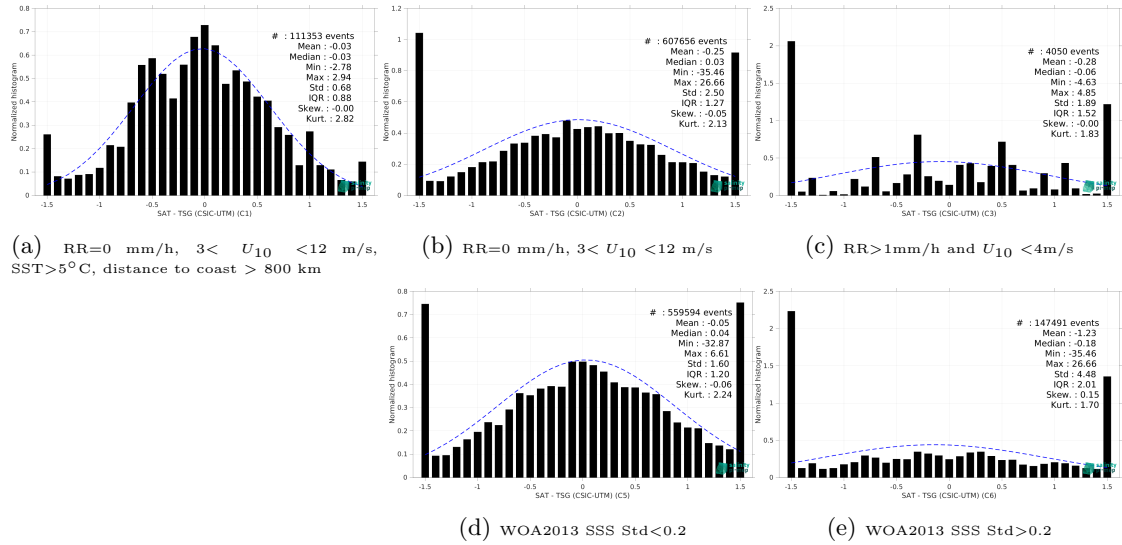
Figure 13: Normalized histogram of \Delta SSS (SMOS SSS L2Q v331 - With FLAG (CMEMS-CATDS-CPDC) - TSG (CSIC-UTM)) for 5 different subdatasets corresponding to: RR=0 mm/h, 3 < U_{10} < 12 m/s, SST>5°C, distance to coast > 800 km (a), RR=0 mm/h, 3 < U_{10} < 12 m/s (b), RR>1mm/h and U_{10} < 4 m/s (c), WOA2013 SSS Std<0.2 (d), WOA2013 SSS Std>0.2 (e).
