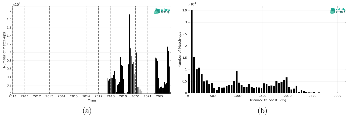
Figure 2: Number of match-ups between Saildrone and SMOS SSS L2Q v331 - With FLAG (CMEMS-CATDS-CPDC) SSS as a function of time (a) and as function of the distance to coast (b) over the Mid-Low Latitudes 45N-45S Pi-MEP region and for the full satellite product period.
