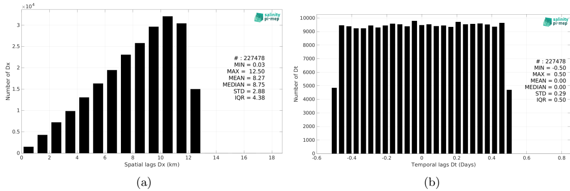
Figure 6: Histograms of the spatial (a) and temporal (b) lags between the location/time of the Saildrone measurement and the date of the corresponding SMOS SSS L2Q v331 - With FLAG (CMEMS-CATDS-CPDC) SSS pixel.
