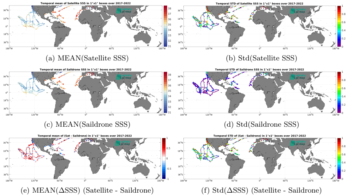
Figure 7: Temporal mean (left) and Std (right) of SSS from SMOS SSS L2Q v331 - With FLAG (CMEMS-CATDS-CPDC) (top), Saildrone (middle), and of \Delta SSS (Satellite - Saildrone). Only match-up pairs are used to generate these maps.
