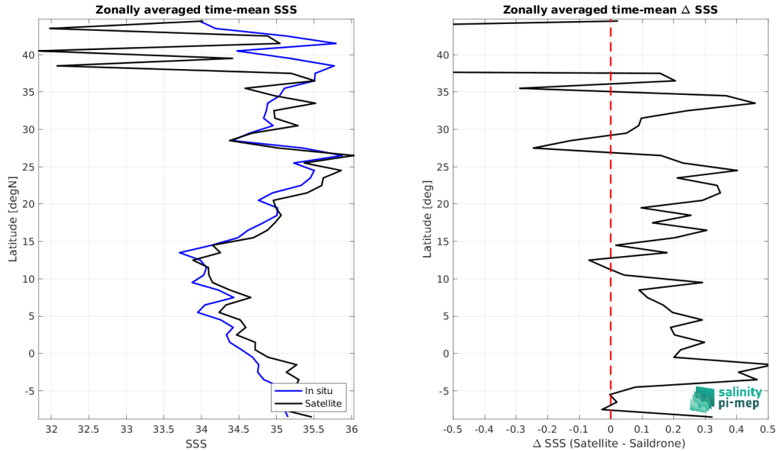
Figure 9: Left panel: Zonal mean SSS from SMOS SSS L2Q v331 - With FLAG (CMEMS-CATDS-CPDC) satellite product (black) and from Saildrone (blue). Right panel: Zonal mean of \Delta SSS (Satellite - Saildrone) for all the collected Pi-MEP match-up pairs estimated over the full satellite product period.
