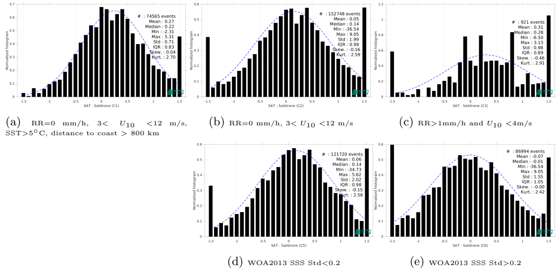
Figure 15: Normalized histogram of \Delta SSS (SMOS SSS L2Q v331 - With FLAG (CMEMS-CATDS-CPDC) - Salldrone) for 5 different subdatasets corresponding to: RR=0 mm/h, 3 < U_{10} < 12 m/s, SST > 5°C, distance to coast > 800 km (a), RR=0 mm/h, 3 < U_{10} < 12 m/s (b), RR > 1mm/h and U_{10} < 4 m/s (c), WOA2013 SSS Std < 0.2 (d), WOA2013 SSS Std > 0.2 (e).
