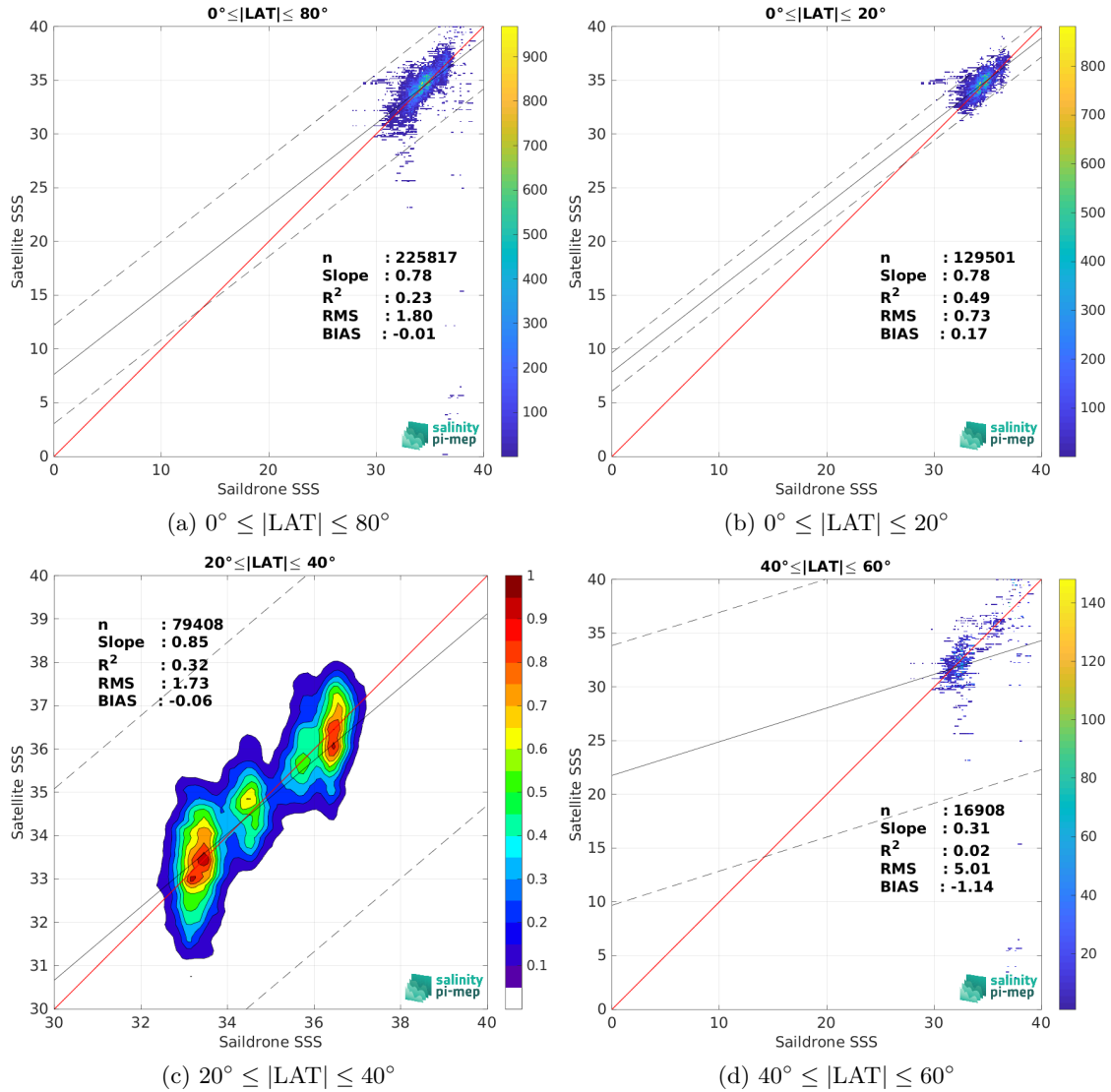
Figure 10: Contour maps of the concentration of SMOS SSS L2Q v331 - With FLAG (CMEMS-CATDS-CPDC) SSS (y-axis) versus Saildrone SSS (x-axis) at match-up pairs for different latitude bands. For each plot, the red line shows x=y . The black thin and dashed lines indicate a linear fit through the data cloud and the \pm 95\% confidence levels, respectively. The number match-up pairs n , the slope and R^2 coefficient of the linear fit, the root mean square (RMS) and the mean bias between satellite and in situ data are indicated for each latitude band in each plots.
