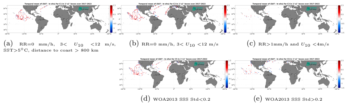
Figure 14: Temporal mean gridded over spatial boxes of size 1^\circ \times 1^\circ of \Delta SSS (SMOS SSS L2Q v331 - With FLAG (CMEMS-CATDS-CPDC) - Saildrone) for 5 different subdatasets corresponding to: RR=0 mm/h, 3 < U_{10} < 12 m/s, SST > 5°C, distance to coast > 800 km (a), RR=0 mm/h, 3 < U_{10} < 12 m/s (b), RR > 1mm/h and U_{10} < 4 m/s (c), WOA2013 SSS Std < 0.2 (d), WOA2013 SSS Std > 0.2 (e).
