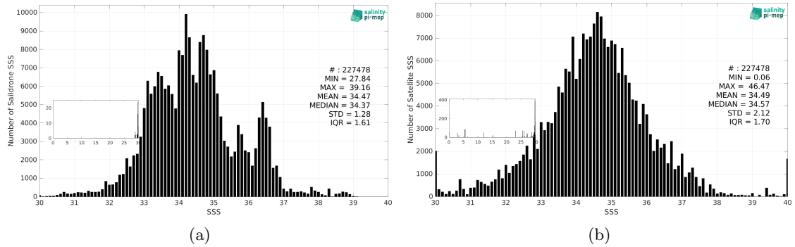
Figure 3: Histograms of SSS from Saildrone (a) and SMOS SSS L2Q v331 - With FLAG (CMEMS-CATDS-CPDC) (b) considering all match-up pairs per bins of 0.1 over the Mid-Low Latitudes 45N-45S Pi-MEP region and for the full satellite product period.
