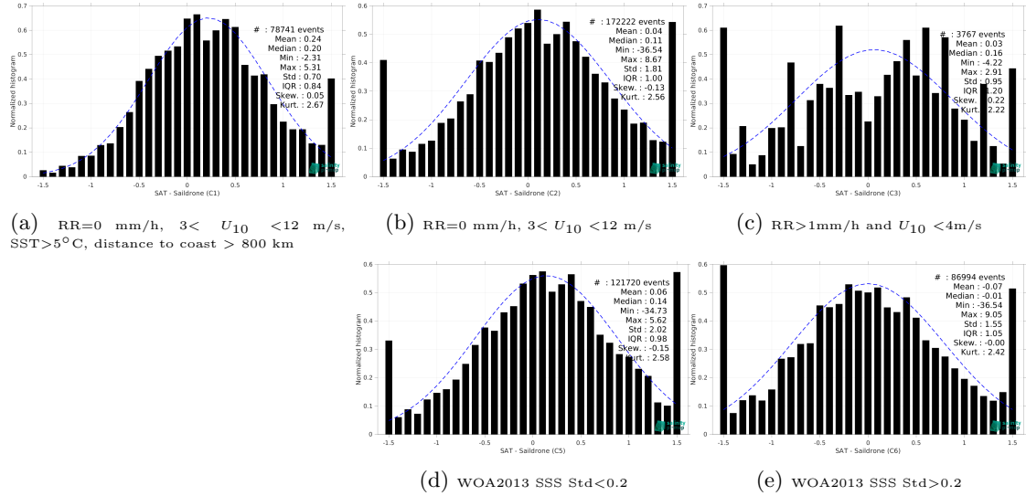
Figure 13: Normalized histogram of \Delta SSS (SMOS SSS L2Q v331 - With FLAG (CMEMS-CATDS-CPDC) - Sairdrone) for 5 different subdatasets corresponding to: RR=0 mm/h, 3 < U_{10} < 12 m/s, SST > 5°C, distance to coast > 800 km (a), RR=0 mm/h, 3 < U_{10} < 12 m/s (b), RR > 1mm/h and U_{10} < 4 m/s (c), WOA2013 SSS Std < 0.2 (d), WOA2013 SSS Std > 0.2 (e).
