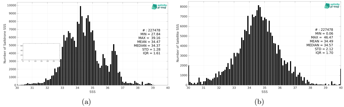
Figure 2: Histograms of SSS from Saildrone (a) and SMOS SSS L2Q v331 - With FLAG (CMEMS-CATDS-CPDC) (b) considering all match-up pairs per bins of 0.1 over the Mid-Low Latitudes 45N-45S Pi-MEP region and for the full satellite product period.
