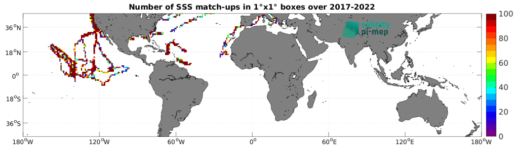
Figure 4: Number of SSS match-ups between Saildrone SSS and the SMOS SSS L2Q v331 - With FLAG (CMEMS-CATDS-CPDC) SSS product for the Mid-Low Latitudes 45N-45S Pi-MEP region over 1^\circ \times 1^\circ boxes and for the full satellite product period.
