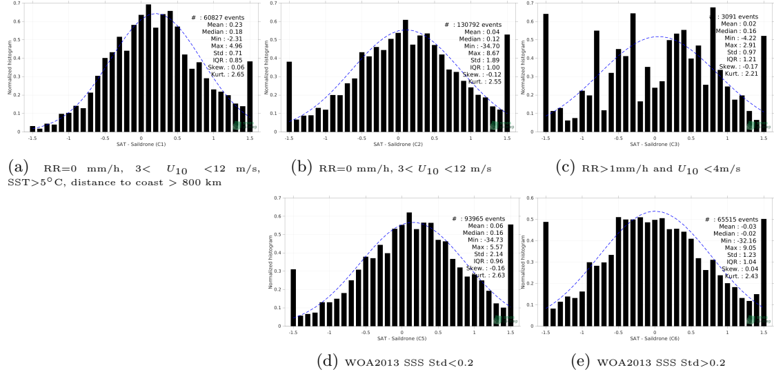
Figure 13: Normalized histogram of \Delta SSS (SMOS SSS L2Q v331 - With FLAG (CMEMS-CATDS-CPDC) - Sairdrone) for 5 different subdatasets corresponding to: RR=0 mm/h, 3 < U_{10} < 12 m/s, SST>5°C, distance to coast > 800 km (a), RR=0 mm/h, 3 < U_{10} < 12 m/s (b), RR>1mm/h and U_{10} < 4 m/s (c), WOA2013 SSS Std<0.2 (d), WOA2013 SSS Std>0.2 (e).
