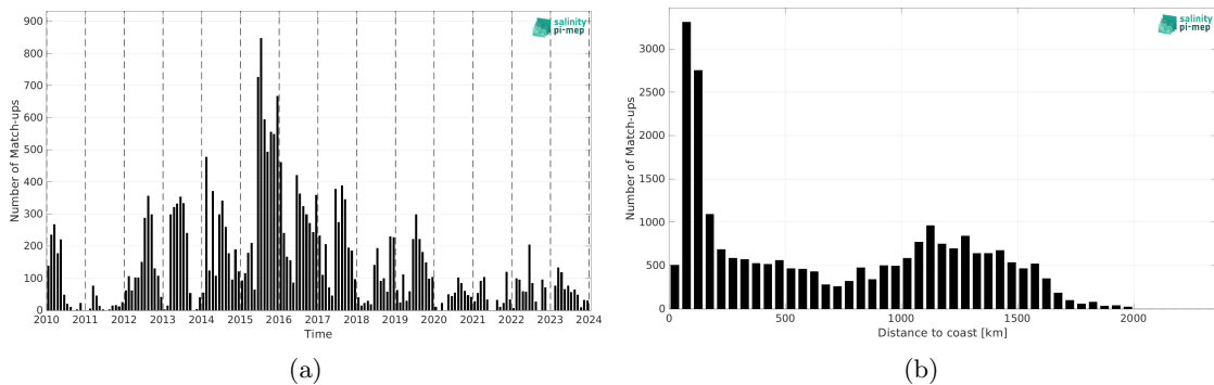
Figure 2: Number of match-ups between Marine mammals and SMOS SSS L2Q v331 - With FLAG (CMEMS-CATDS-CPDC) SSS as a function of time (a) and as function of the distance to coast (b) over the Mid-Low Latitudes 45N-45S Pi-MEP region and for the full satellite product period.
