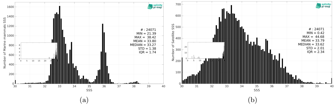
Figure 3: Histograms of SSS from Marine mammals (a) and SMOS SSS L2Q v331 - With FLAG (CMEMS-CATDS-CPDC) (b) considering all match-up pairs per bins of 0.1 over the Mid-Low Latitudes 45N-45S Pi-MEP region and for the full satellite product period.
