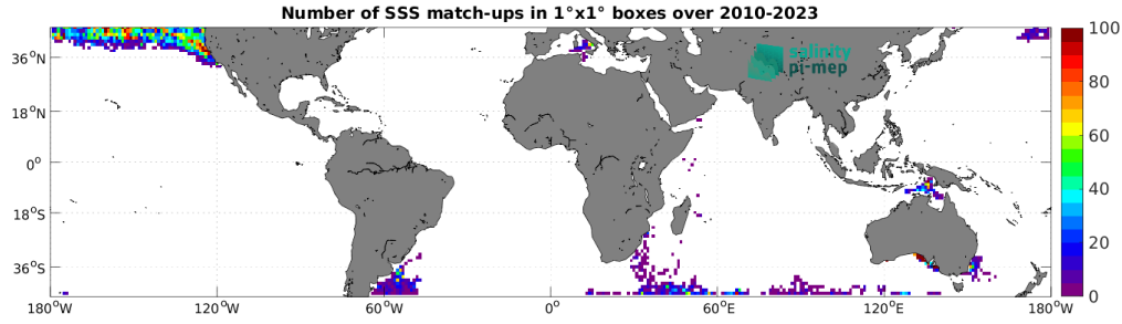
Figure 5: Number of SSS match-ups between Marine mammals SSS and the SMOS SSS L2Q v331 - With FLAG (CMEMS-CATDS-CPDC) SSS product for the Mid-Low Latitudes 45N-45S Pi-MEP region over 1^\circ \times 1^\circ boxes and for the full satellite product period.
