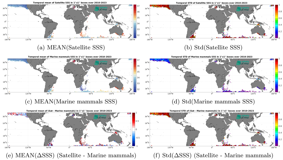
Figure 7: Temporal mean (left) and Std (right) of SSS from SMOS SSS L2Q v331 - With FLAG (CMEMS-CATDS-CPDC) (top), Marine mammals (middle), and of \Delta SSS (Satellite - Marine mammals). Only match-up pairs are used to generate these maps.
