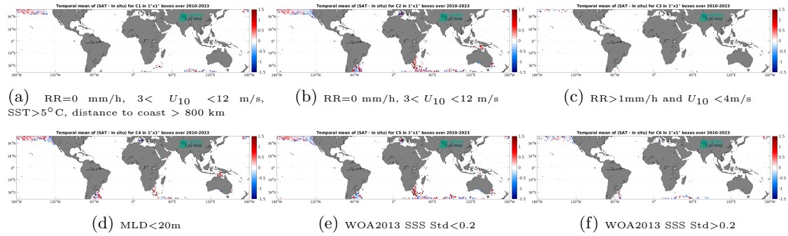
Figure 14: Temporal mean gridded over spatial boxes of size 1^\circ \times 1^\circ of \Delta SSS (SMOS SSS L2Q v331 - With FLAG (CMEMS-CATDS-CPDC) - Marine mammals) for 6 different subdatasets corresponding to:RR=0 mm/h, 3 < U_{10} < 12 m/s, SST >5^\circ\text{C} , distance to coast > 800 km (a), RR=0 mm/h, 3 < U_{10} < 12 m/s (b), RR >1 mm/h and U_{10} < 4 m/s (c),MLD <20 m (d),WOA2013 SSS Std <0.2 (e),WOA2013 SSS Std >0.2 (f).
