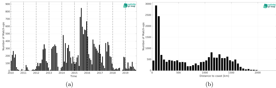
Figure 1: Number of match-ups between Marine mammals and SMOS SSS L2Q v331 - With FLAG (CMEMS-CATDS-CPDC) SSS as a function of time (a) and as function of the distance to coast (b) over the Mid-Low Latitudes 45N-45S Pi-MEP region and for the full satellite product period.
