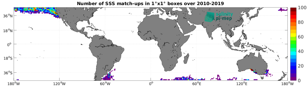
Figure 4: Number of SSS match-ups between Marine mammals SSS and the SMOS SSS L2Q v331 - With FLAG (CMEMS-CATDS-CPDC) SSS product for the Mid-Low Latitudes 45N-45S Pi-MEP region over 1^{\circ} \times 1^{\circ} boxes and for the full satellite product period.
