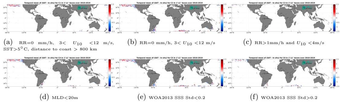
Figure 12: Temporal mean gridded over spatial boxes of size 1^{\circ}\times 1^{\circ} of \Delta\text{SSS} (SMOS SSS L2Q v331 - With FLAG (CMEMS-CATDS-CPDC) - Marine mammals) for 6 different subdatasets corresponding to: \text{RR}=0 mm/h, 3 < U_{10} < 12 m/s, \text{SST} > 5^{\circ}\text{C} , distance to coast > 800 km (a), \text{RR}=0 mm/h, 3 < U_{10} < 12 m/s (b), \text{RR} > 1 mm/h and U_{10} < 4 m/s (c), \text{MLD} < 20\text{m} (d), WOA2013 SSS Std < 0.2 (e), WOA2013 SSS Std > 0.2 (f).
