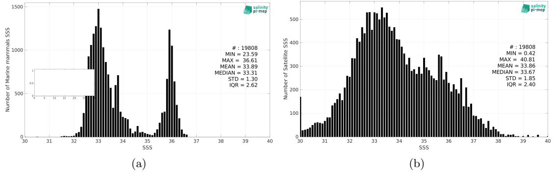
Figure 2: Histograms of SSS from Marine mammals (a) and SMOS SSS L2Q v331 - With FLAG (CMEMS-CATDS-CPDC) (b) considering all match-up pairs per bins of 0.1 over the Mid-Low Latitudes 45N-45S Pi-MEP region and for the full satellite product period.
