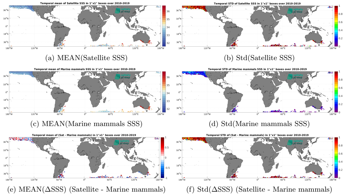
Figure 6: Temporal mean (left) and Std (right) of SSS from SMOS SSS L2Q v331 - With FLAG (CMEMS-CATDS-CPDC) (top), Marine mammals (middle), and of \Delta SSS (Satellite - Marine mammals). Only match-up pairs are used to generate these maps.
