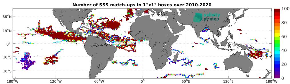
Figure 4: Number of SSS match-ups between Surface drifters SSS and the SMOS SSS L2Q v331 - With FLAG (CMEMS-CATDS-CPDC) SSS product for the Mid-Low Latitudes 45N-45S Pi-MEP region over 1^\circ \times 1^\circ boxes and for the full satellite product period.
