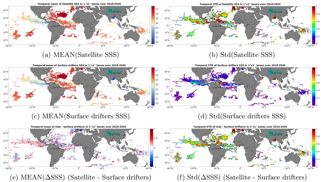
Figure 6: Temporal mean (left) and Std (right) of SSS from SMOS SSS L2Q v331 - With FLAG (CMEMS-CATDS-CPDC) (top), Surface drifters (middle), and of \Delta SSS (Satellite - Surface drifters). Only match-up pairs are used to generate these maps.
