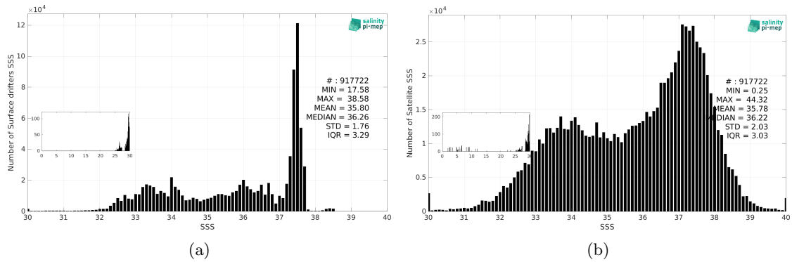
Figure 3: Histograms of SSS from Surface drifters (a) and SMOS SSS L2Q v331 - With FLAG (CMEMS-CATDS-CPDC) (b) considering all match-up pairs per bins of 0.1 over the Mid-Low Latitudes 45N-45S Pi-MEP region and for the full satellite product period.
