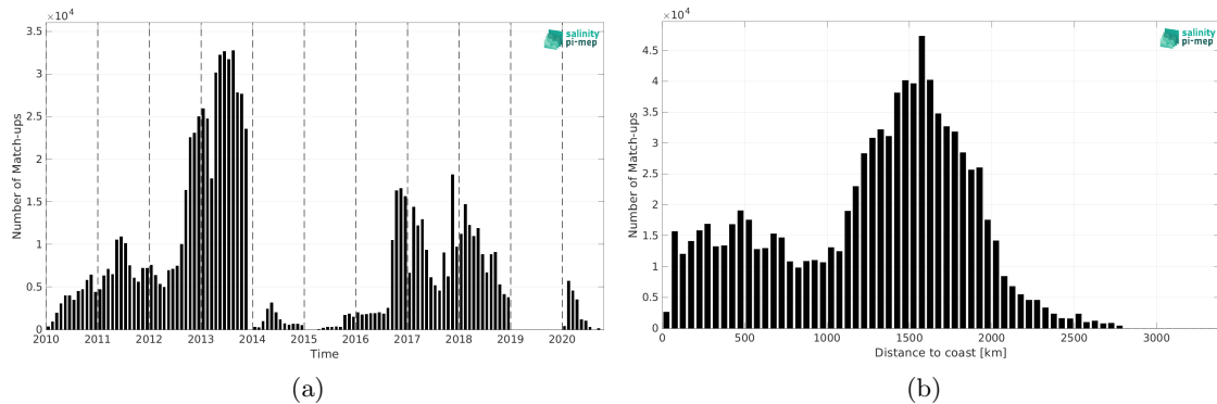
Figure 2: Number of match-ups between Surface drifters and SMOS SSS L2Q v331 - With FLAG (CMEMS-CATDS-CPDC) SSS as a function of time (a) and as function of the distance to coast (b) over the Mid-Low Latitudes 45N-45S Pi-MEP region and for the full satellite product period.
