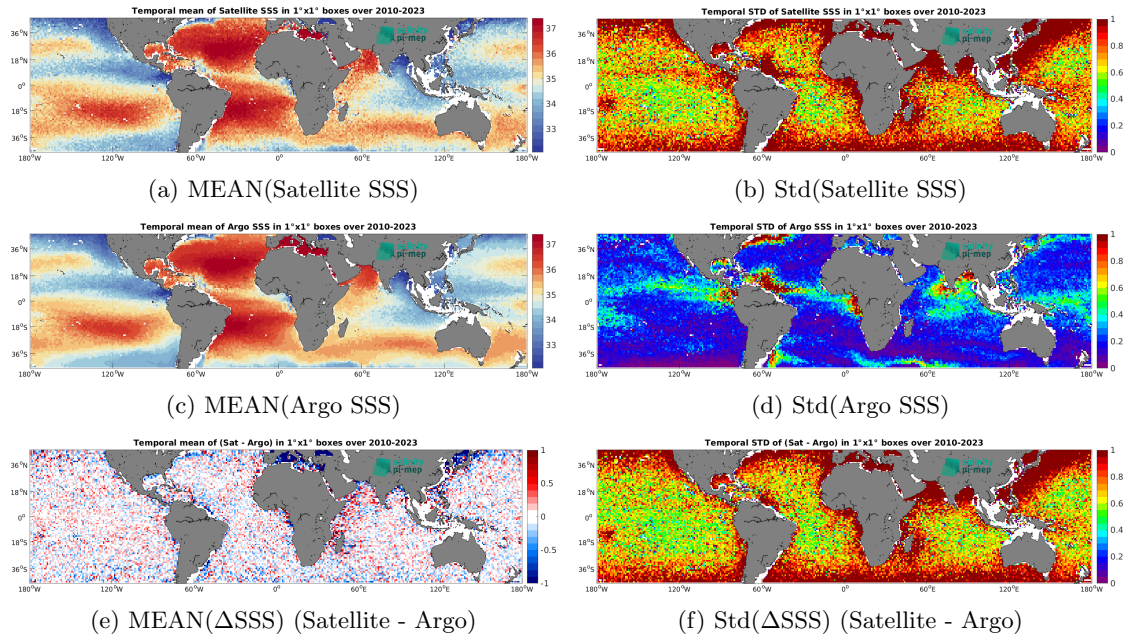
Figure 6: Temporal mean (left) and Std (right) of SSS from SMOS SSS L2Q v331 - With FLAG (CMEMS-CATDS-CPDC) (top), Argo (middle), and of \Delta SSS (Satellite - Argo). Only match-up pairs are used to generate these maps.
