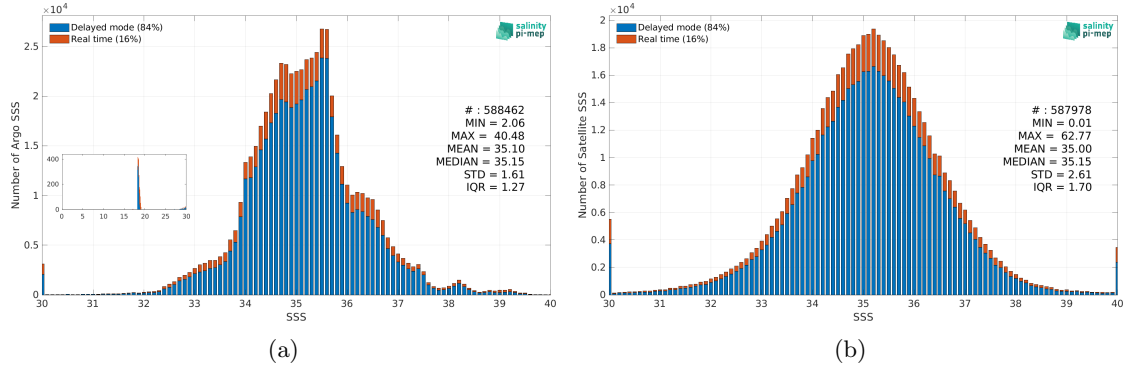
Figure 2: Histograms of SSS from Argo (a) and SMOS SSS L2Q v331 - With FLAG (CMEMS-CATDS-CPDC) (b) considering all match-up pairs per bins of 0.1 over the Mid-Low Latitudes 45N-45S Pi-MEP region and for the full satellite product period.
