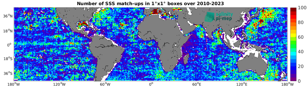
Figure 4: Number of SSS match-ups between Argo SSS and the SMOS SSS L2Q v331 - With FLAG (CMEMS-CATDS-CPDC) SSS product for the Mid-Low Latitudes 45N-45S Pi-MEP region over 1^\circ \times 1^\circ boxes and for the full satellite product period.
