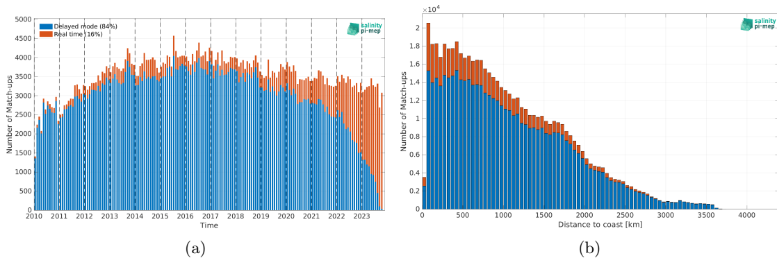
Figure 1: Number of match-ups between Argo and SMOS SSS L2Q v331 - With FLAG (CMEMS-CATDS-CPDC) SSS as a function of time (a) and as function of the distance to coast (b) over the Mid-Low Latitudes 45N-45S Pi-MEP region and for the full satellite product period.
