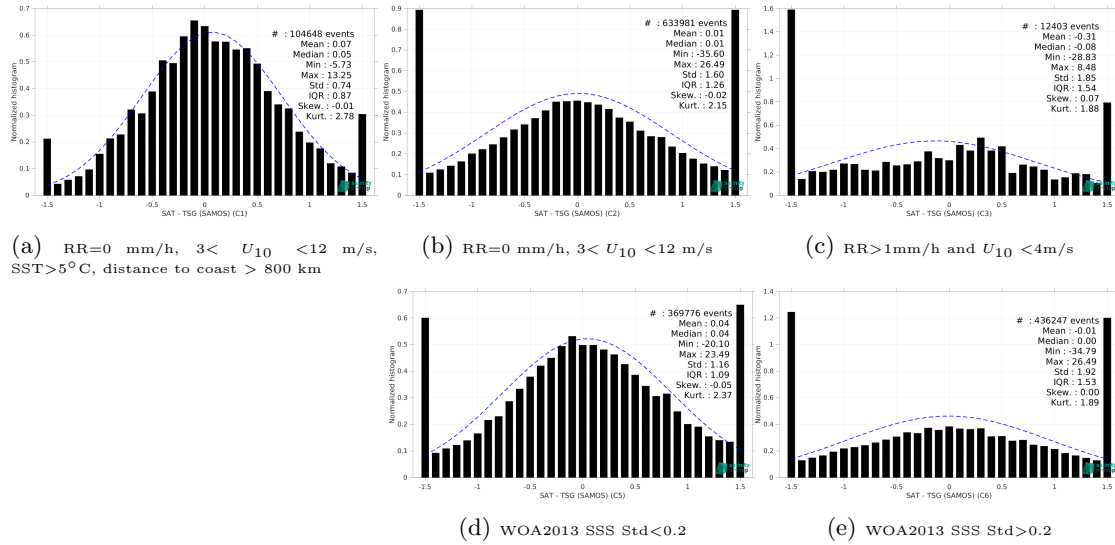
Figure 13: Normalized histogram of \Delta SSS (SMOS SSS L2Q v331 - No FLAG (CMEMS-CATDS-CPDC) - TSG (SAMOS)) for 5 different subdatasets corresponding to: RR=0 mm/h, 3 < U_{10} < 12 m/s, SST > 5°C, distance to coast > 800 km (a), RR=0 mm/h, 3 < U_{10} < 12 m/s (b), RR > 1mm/h and U_{10} < 4 m/s (c), WOA2013 SSS Std < 0.2 (d), WOA2013 SSS Std > 0.2 (e).
