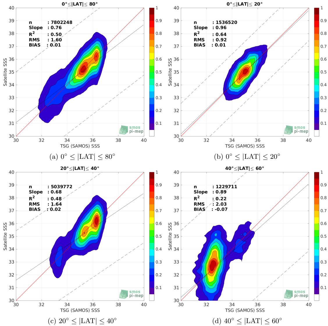
Figure 9: Contour maps of the concentration of SMOS SSS L2Q v331 - No FLAG (CMEMS-CATDS-CPDC) SSS (y-axis) versus TSG (SAMOS) SSS (x-axis) at match-up pairs for different latitude bands. For each plot, the red line shows x=y . The black thin and dashed lines indicate a linear fit through the data cloud and the \pm 95\% confidence levels, respectively. The number match-up pairs n , the slope and R^2 coefficient of the linear fit, the root mean square (RMS) and the mean bias between satellite and in situ data are indicated for each latitude band in each plots.
