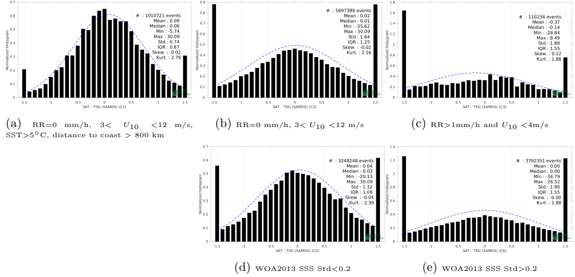
Figure 13: Normalized histogram of \Delta SSS (SMOS SSS L2Q v331 - No FLAG (CMEMS-CATDS-CPDC) - TSG (SAMOS)) for 5 different subdatasets corresponding to: RR=0 mm/h, 3 < U_{10} < 12 m/s, SST > 5°C, distance to coast > 800 km (a), RR=0 mm/h, 3 < U_{10} < 12 m/s (b), RR > 1mm/h and U_{10} < 4 m/s (c), WOA2013 SSS Std < 0.2 (d), WOA2013 SSS Std > 0.2 (e).
