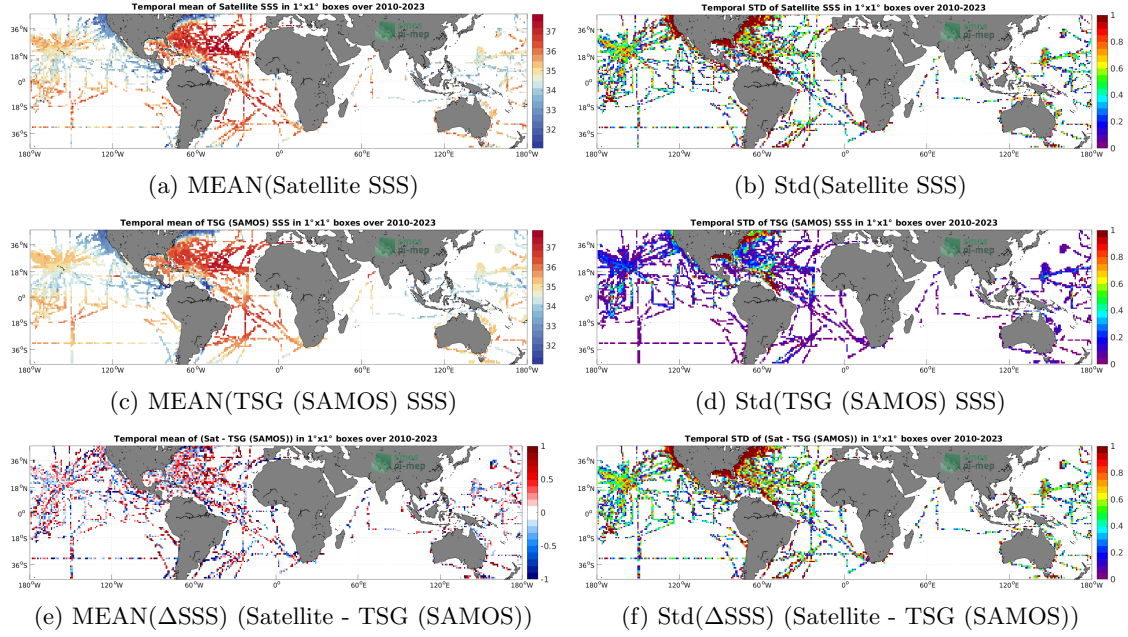
Figure 6: Temporal mean (left) and Std (right) of SSS from SMOS SSS L2Q v331 - No FLAG (CMEMS-CATDS-CPDC) (top), TSG (SAMOS) (middle), and of \Delta SSS (Satellite - TSG (SAMOS)). Only match-up pairs are used to generate these maps.
