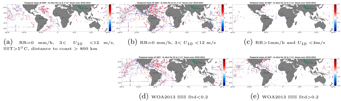
Figure 12: Temporal mean gridded over spatial boxes of size 1^\circ \times 1^\circ of \Delta SSS (SMOS SSS L2Q v331 - No FLAG (CMEMS-CATDS-CPDC) - TSG (SAMOS)) for 5 different subdatasets corresponding to:RR=0 mm/h, 3 < U_{10} < 12 m/s, SST >5^\circ C, distance to coast > 800 km (a), RR=0 mm/h, 3 < U_{10} < 12 m/s (b), RR >1 mm/h and U_{10} < 4 m/s (c), WOA2013 SSS Std <0.2 (d), WOA2013 SSS Std >0.2 (e).
