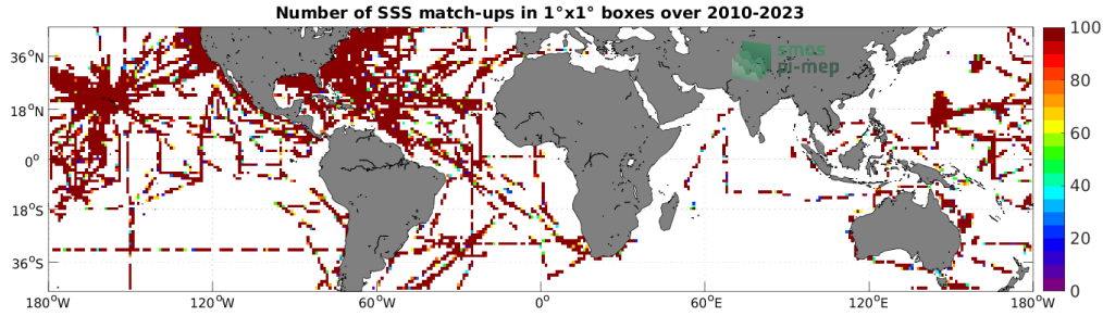
Figure 4: Number of SSS match-ups between TSG (SAMOS) SSS and the SMOS SSS L2Q v331 - No FLAG (CMEMS-CATDS-CPDC) SSS product for the Mid-Low Latitudes 45N-45S Pi-MEP region over 1^\circ \times 1^\circ boxes and for the full satellite product period.
