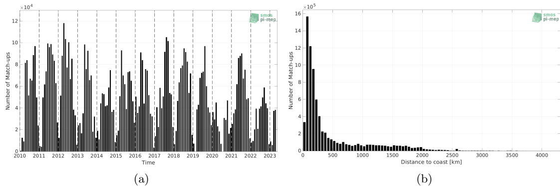
Figure 1: Number of match-ups between TSG (SAMOS) and SMOS SSS L2Q v331 - No FLAG (CMEMS-CATDS-CPDC) SSS as a function of time (a) and as function of the distance to coast (b) over the Mid-Low Latitudes 45N-45S Pi-MEP region and for the full satellite product period.
