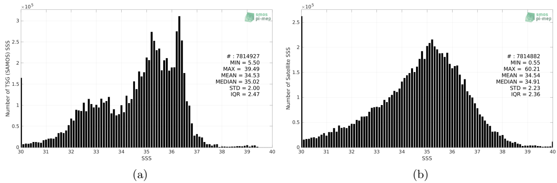
Figure 2: Histograms of SSS from TSG (SAMOS) (a) and SMOS SSS L2Q v331 - No FLAG (CMEMS-CATDS-CPDC) (b) considering all match-up pairs per bins of 0.1 over the Mid-Low Latitudes 45N-45S Pi-MEP region and for the full satellite product period.
