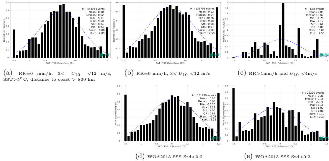
Figure 15: Normalized histogram of \Delta\text{SSS} (SMOS SSS L2Q v331 - No FLAG (CMEMS-CATDS-CPDC) - TSG (Polarstern)) for 5 different subdatasets corresponding to: RR=0 mm/h, 3 < U_{10} < 12 m/s, SST>5°C, distance to coast > 800 km (a), RR=0 mm/h, 3 < U_{10} < 12 m/s (b), RR>1mm/h and U_{10} < 4 m/s (c), WOA2013 SSS Std<0.2 (d), WOA2013 SSS Std>0.2 (e).
