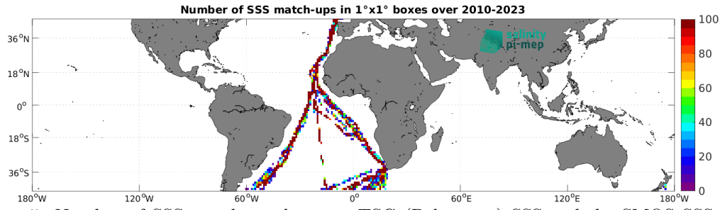
Figure 5: Number of SSS match-ups between TSG (Polarstern) SSS and the SMOS SSS L2Q v331 - No FLAG (CMEMS-CATDS-CPDC) SSS product for the Mid-Low Latitudes 45N-45S Pi-MEP region over 1^\circ \times 1^\circ boxes and for the full satellite product period.
