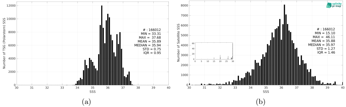
Figure 3: Histograms of SSS from TSG (Polarstern) (a) and SMOS SSS L2Q v331 - No FLAG (CMEMS-CATDS-CPDC) (b) considering all match-up pairs per bins of 0.1 over the Mid-Low Latitudes 45N-45S Pi-MEP region and for the full satellite product period.
