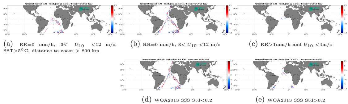
Figure 14: Temporal mean gridded over spatial boxes of size 1^\circ \times 1^\circ of \Delta SSS (SMOS SSS L2Q v331 - No FLAG (CMEMS-CATDS-CPDC) - TSG (Polarstern)) for 5 different subdatasets corresponding to: RR=0 mm/h, 3 < U_{10} < 12 m/s, SST > 5°C, distance to coast > 800 km (a), RR=0 mm/h, 3 < U_{10} < 12 m/s (b), RR > 1mm/h and U_{10} < 4 m/s (c), WOA2013 SSS Std < 0.2 (d), WOA2013 SSS Std > 0.2 (e).
