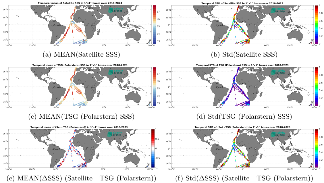
Figure 7: Temporal mean (left) and Std (right) of SSS from SMOS SSS L2Q v331 - No FLAG (CMEMS-CATDS-CPDC) (top), TSG (Polarstern) (middle), and of \Delta SSS (Satellite - TSG (Polarstern)). Only match-up pairs are used to generate these maps.
