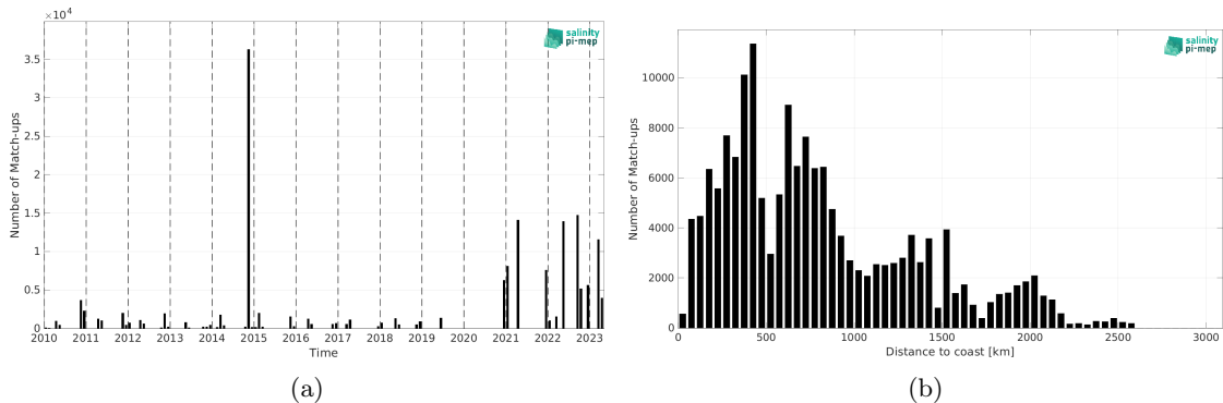
Figure 2: Number of match-ups between TSG (Polarstern) and SMOS SSS L2Q v331 - No FLAG (CMEMS-CATDS-CPDC) SSS as a function of time (a) and as function of the distance to coast (b) over the Mid-Low Latitudes 45N-45S Pi-MEP region and for the full satellite product period.
