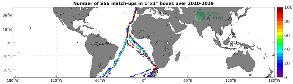
Figure 4: Number of SSS match-ups between TSG (Polarstern) SSS and the SMOS SSS L2Q v331 - No FLAG (CMEMS-CATDS-CPDC) SSS product for the Mid-Low Latitudes 45N-45S Pi-MEP region over 1^\circ \times 1^\circ boxes and for the full satellite product period.
