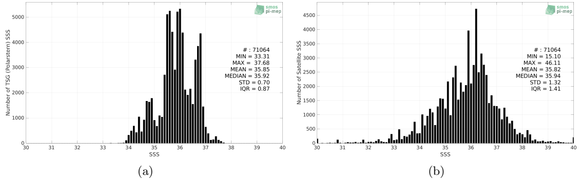
Figure 2: Histograms of SSS from TSG (Polarstern) (a) and SMOS SSS L2Q v331 - No FLAG (CMEMS-CATDS-CPDC) (b) considering all match-up pairs per bins of 0.1 over the Mid-Low Latitudes 45N-45S Pi-MEP region and for the full satellite product period.
