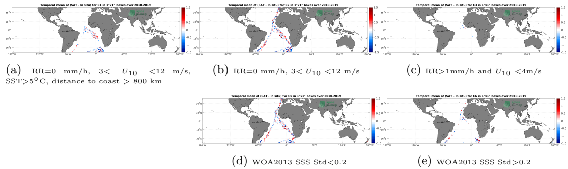
Figure 12: Temporal mean gridded over spatial boxes of size 1^\circ \times 1^\circ of \Delta SSS (SMOS SSS L2Q v331 - No FLAG (CMEMS-CATDS-CPDC) - TSG (Polarstern)) for 5 different subdatasets corresponding to:RR=0 mm/h, 3 < U_{10} < 12 m/s, SST >5^\circ C, distance to coast > 800 km (a), RR=0 mm/h, 3 < U_{10} < 12 m/s (b), RR >1 mm/h and U_{10} < 4 m/s (c), WOA2013 SSS Std <0.2 (d), WOA2013 SSS Std >0.2 (e).
