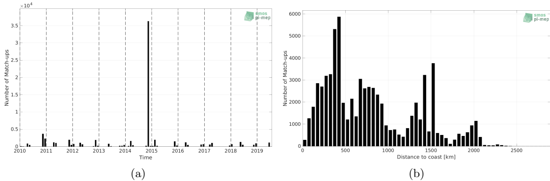
Figure 1: Number of match-ups between TSG (Polarstern) and SMOS SSS L2Q v331 - No FLAG (CMEMS-CATDS-CPDC) SSS as a function of time (a) and as function of the distance to coast (b) over the Mid-Low Latitudes 45N-45S Pi-MEP region and for the full satellite product period.
