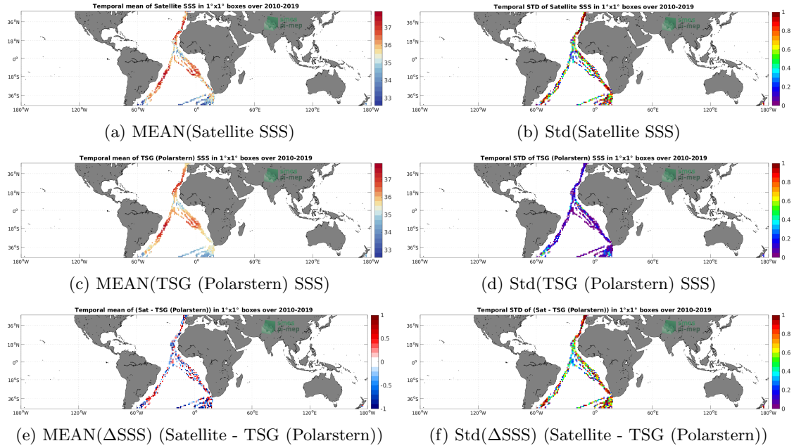
Figure 6: Temporal mean (left) and Std (right) of SSS from SMOS SSS L2Q v331 - No FLAG (CMEMS-CATDS-CPDC) (top), TSG (Polarstern) (middle), and of \Delta SSS (Satellite - TSG (Polarstern)). Only match-up pairs are used to generate these maps.
