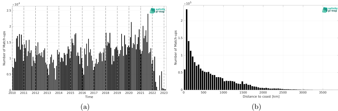
Figure 2: Number of match-ups between TSG (LEGOS-DM) and SMOS SSS L2Q v331 - No FLAG (CMEMS-CATDS-CPDC) SSS as a function of time (a) and as function of the distance to coast (b) over the Mid-Low Latitudes 45N-45S Pi-MEP region and for the full satellite product period.
