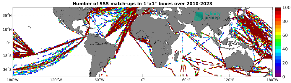
Figure 5: Number of SSS match-ups between TSG (LEGOS-DM) SSS and the SMOS SSS L2Q v331 - No FLAG (CMEMS-CATDS-CPDC) SSS product for the Mid-Low Latitudes 45N-45S Pi-MEP region over 1^\circ \times 1^\circ boxes and for the full satellite product period.
