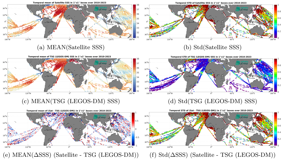
Figure 7: Temporal mean (left) and Std (right) of SSS from SMOS SSS L2Q v331 - No FLAG (CMEMS-CATDS-CPDC) (top), TSG (LEGOS-DM) (middle), and of \Delta SSS (Satellite - TSG (LEGOS-DM)). Only match-up pairs are used to generate these maps.
