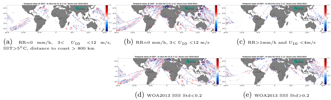
Figure 14: Temporal mean gridded over spatial boxes of size 1^\circ \times 1^\circ of \Delta\text{SSS} (SMOS SSS L2Q v331 - No FLAG (CMEMS-CATDS-CPDC) - TSG (LEGOS-DM)) for 5 different subdatasets corresponding to:RR=0 mm/h, 3 < U_{10} < 12 m/s, SST>5°C, distance to coast > 800 km (a), RR=0 mm/h, 3 < U_{10} < 12 m/s (b), RR>1mm/h and U_{10} < 4 m/s (c), WOA2013 SSS Std<0.2 (d), WOA2013 SSS Std>0.2 (e).
