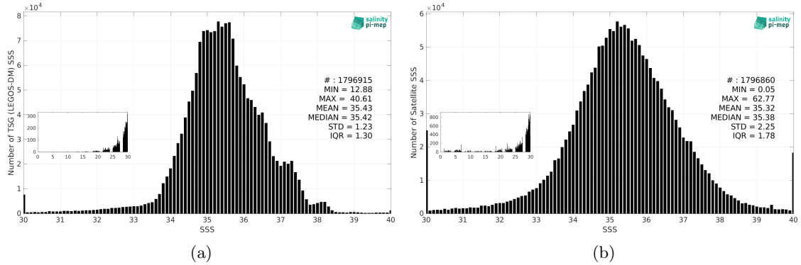
Figure 3: Histograms of SSS from TSG (LEGOS-DM) (a) and SMOS SSS L2Q v331 - No FLAG (CMEMS-CATDS-CPDC) (b) considering all match-up pairs per bins of 0.1 over the Mid-Low Latitudes 45N-45S Pi-MEP region and for the full satellite product period.
