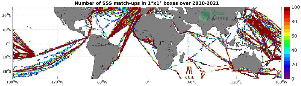
Figure 4: Number of SSS match-ups between TSG (LEGOS-DM) SSS and the SMOS SSS L2Q v331 - No FLAG (CMEMS-CATDS-CPDC) SSS product for the Mid-Low Latitudes 45N-45S Pi-MEP region over 1^\circ \times 1^\circ boxes and for the full satellite product period.
