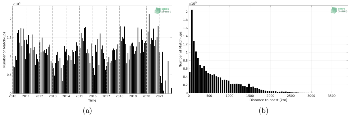
Figure 1: Number of match-ups between TSG (LEGOS-DM) and SMOS SSS L2Q v331 - No FLAG (CMEMS-CATDS-CPDC) SSS as a function of time (a) and as function of the distance to coast (b) over the Mid-Low Latitudes 45N-45S Pi-MEP region and for the full satellite product period.
