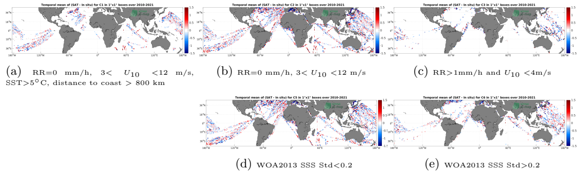
Figure 12: Temporal mean gridded over spatial boxes of size 1^\circ \times 1^\circ of \Delta SSS (SMOS SSS L2Q v331 - No FLAG (CMEMS-CATDS-CPDC) - TSG (LEGOS-DM)) for 5 different subdatasets corresponding to:RR=0 mm/h, 3 < U_{10} < 12 m/s, SST >5^\circ C, distance to coast > 800 km (a), RR=0 mm/h, 3 < U_{10} < 12 m/s (b), RR >1 mm/h and U_{10} < 4 m/s (c), WOA2013 SSS Std <0.2 (d), WOA2013 SSS Std >0.2 (e).
