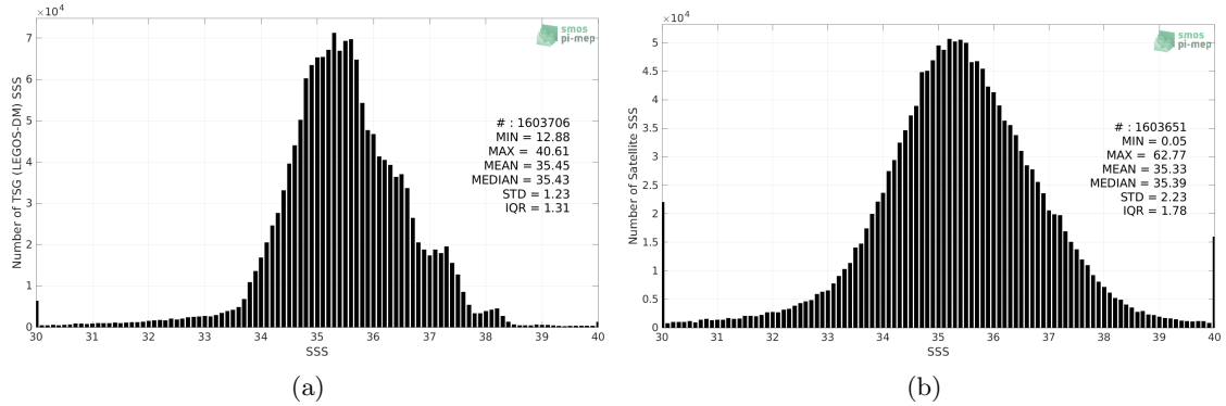
Figure 2: Histograms of SSS from TSG (LEGOS-DM) (a) and SMOS SSS L2Q v331 - No FLAG (CMEMS-CATDS-CPDC) (b) considering all match-up pairs per bins of 0.1 over the Mid-Low Latitudes 45N-45S Pi-MEP region and for the full satellite product period.
