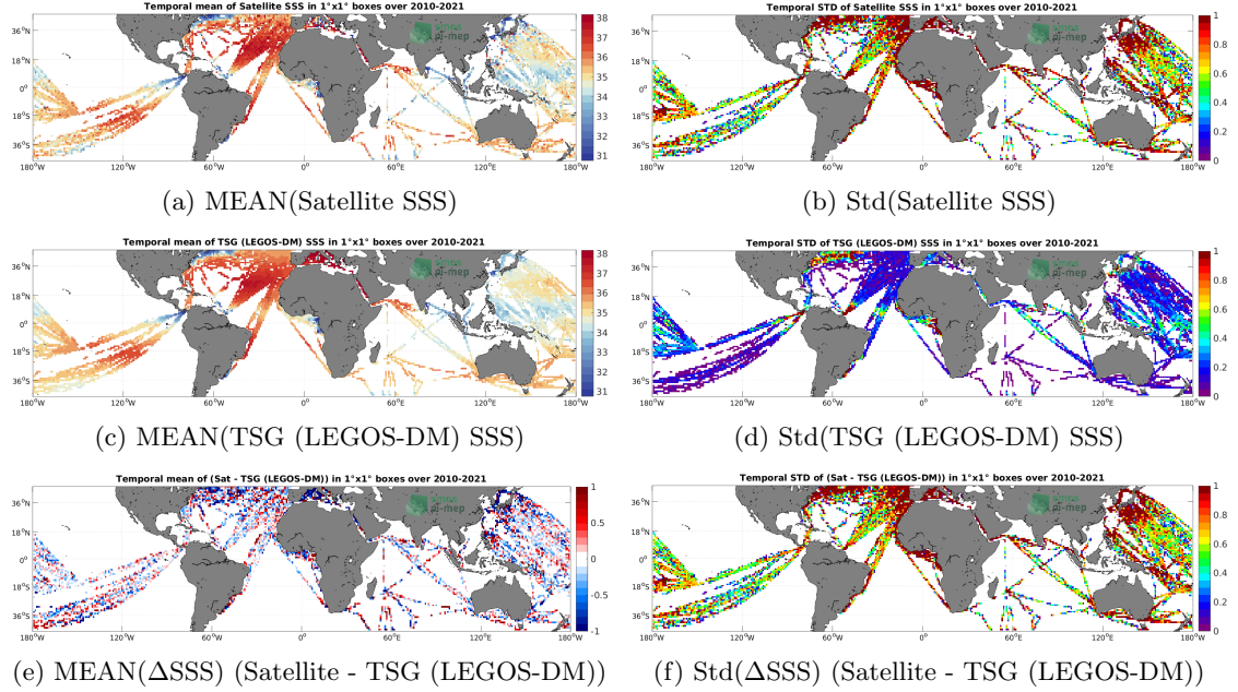
Figure 6: Temporal mean (left) and Std (right) of SSS from SMOS SSS L2Q v331 - No FLAG (CMEMS-CATDS-CPDC) (top), TSG (LEGOS-DM) (middle), and of \Delta SSS (Satellite - TSG (LEGOS-DM)). Only match-up pairs are used to generate these maps.
