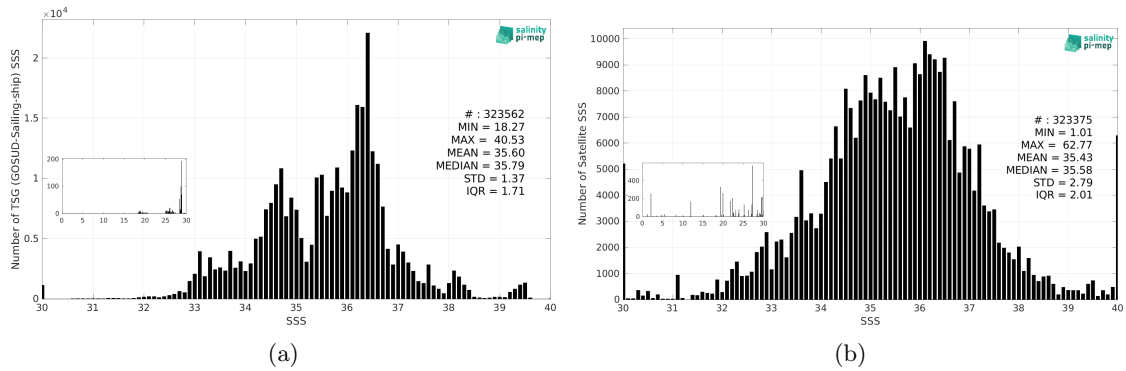
Figure 3: Histograms of SSS from TSG (GOSUD-Sailing-ship) (a) and SMOS SSS L2Q v331 - No FLAG (CMEMS-CATDS-CPDC) (b) considering all match-up pairs per bins of 0.1 over the Mid-Low Latitudes 45N-45S Pi-MEP region and for the full satellite product period.
