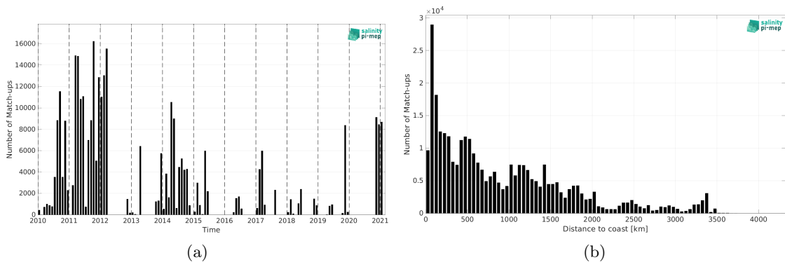
Figure 2: Number of match-ups between TSG (GOSUD-Sailing-ship) and SMOS SSS L2Q v331 - No FLAG (CMEMS-CATDS-CPDC) SSS as a function of time (a) and as function of the distance to coast (b) over the Mid-Low Latitudes 45N-45S Pi-MEP region and for the full satellite product period.
