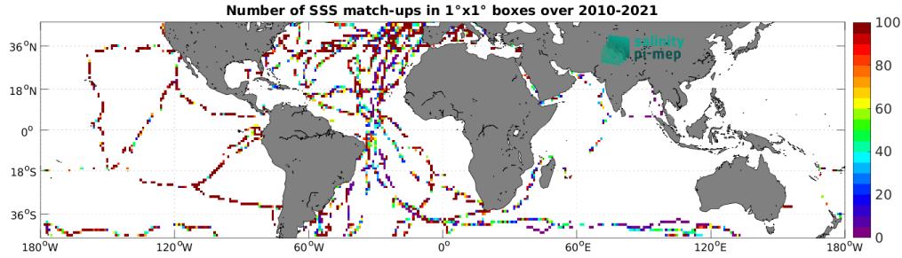
Figure 5: Number of SSS match-ups between TSG (GOSUD-Sailing-ship) SSS and the SMOS SSS L2Q v331 - No FLAG (CMEMS-CATDS-CPDC) SSS product for the Mid-Low Latitudes 45N-45S Pi-MEP region over 1^\circ \times 1^\circ boxes and for the full satellite product period.
