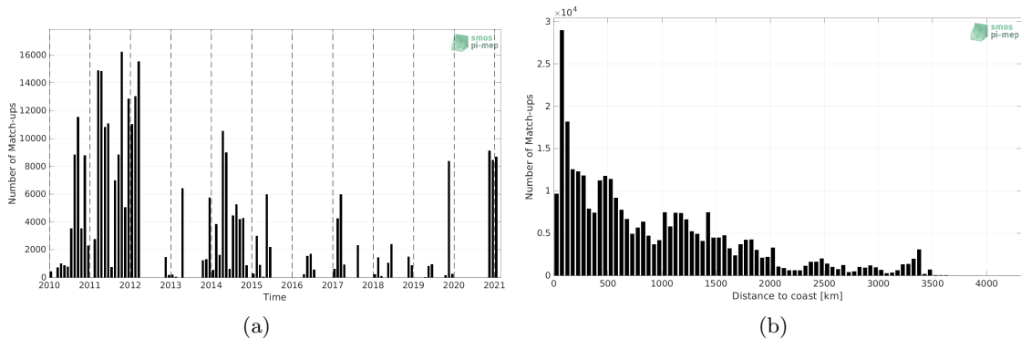
Figure 1: Number of match-ups between TSG (GOSUD-Sailing-ship) and SMOS SSS L2Q v331 - No FLAG (CMEMS-CATDS-CPDC) SSS as a function of time (a) and as function of the distance to coast (b) over the Mid-Low Latitudes 45N-45S Pi-MEP region and for the full satellite product period.
