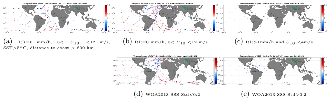
Figure 12: Temporal mean gridded over spatial boxes of size 1^\circ \times 1^\circ of \Delta SSS (SMOS SSS L2Q v331 - No FLAG (CMEMS-CATDS-CPDC) - TSG (GOSUD-Sailing-ship)) for 5 different sub-datasets corresponding to:RR=0 mm/h, 3 < U_{10} < 12 m/s, SST >5^\circ\text{C} , distance to coast > 800 km (a), RR=0 mm/h, 3 < U_{10} < 12 m/s (b), RR >1 mm/h and U_{10} < 4 m/s (c), WOA2013 SSS Std <0.2 (d), WOA2013 SSS Std >0.2 (e).
