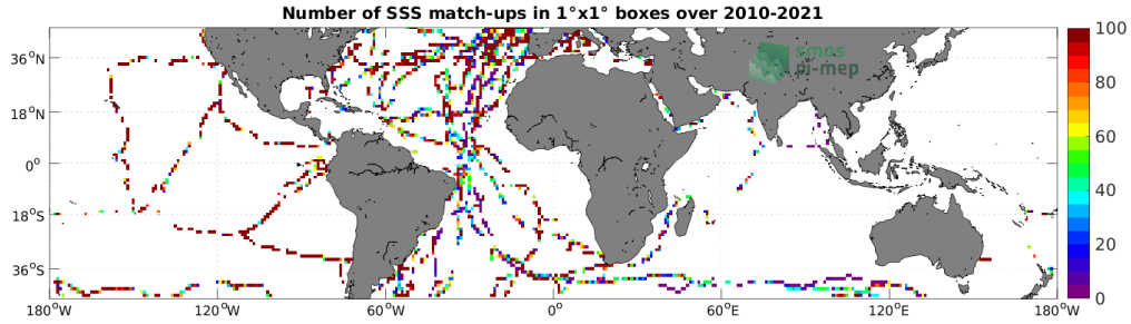
Figure 4: Number of SSS match-ups between TSG (GOSUD-Sailing-ship) SSS and the SMOS SSS L2Q v331 - No FLAG (CMEMS-CATDS-CPDC) SSS product for the Mid-Low Latitudes 45N-45S Pi-MEP region over 1^\circ \times 1^\circ boxes and for the full satellite product period.
