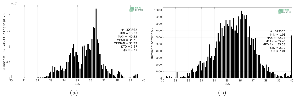
Figure 2: Histograms of SSS from TSG (GOSUD-Sailing-ship) (a) and SMOS SSS L2Q v331 - No FLAG (CMEMS-CATDS-CPDC) (b) considering all match-up pairs per bins of 0.1 over the Mid-Low Latitudes 45N-45S Pi-MEP region and for the full satellite product period.
