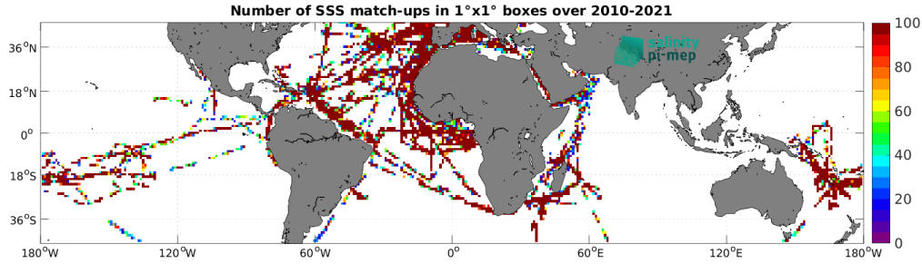
Figure 4: Number of SSS match-ups between TSG (GOSUD-Research-vessel) SSS and the SMOS SSS L2Q v331 - No FLAG (CMEMS-CATDS-CPDC) SSS product for the Mid-Low Latitudes 45N-45S Pi-MEP region over 1^{\circ} \times 1^{\circ} boxes and for the full satellite product period.
