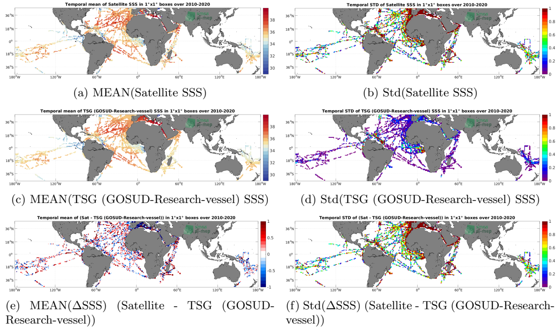
Figure 6: Temporal mean (left) and Std (right) of SSS from SMOS SSS L2Q v331 - No FLAG (CMEMS-CATDS-CPDC) (top), TSG (GOSUD-Research-vessel) (middle), and of \Delta SSS (Satellite - TSG (GOSUD-Research-vessel)). Only match-up pairs are used to generate these maps.
