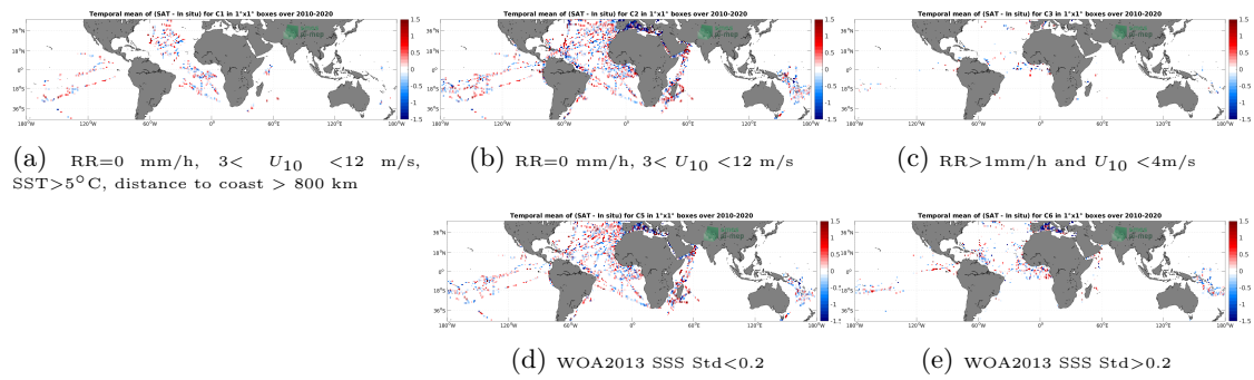
Figure 12: Temporal mean gridded over spatial boxes of size 1^\circ \times 1^\circ of \Delta\text{SSS} (SMOS SSS L2Q v331 - No FLAG (CMEMS-CATDS-CPDC) - TSG (GOSUD-Research-vessel)) for 5 different subdatasets corresponding to: RR=0 mm/h, 3 < U_{10} < 12 m/s, SST > 5°C, distance to coast > 800 km (a), RR=0 mm/h, 3 < U_{10} < 12 m/s (b), RR > 1mm/h and U_{10} < 4 m/s (c), WOA2013 SSS Std < 0.2 (d), WOA2013 SSS Std > 0.2 (e).
