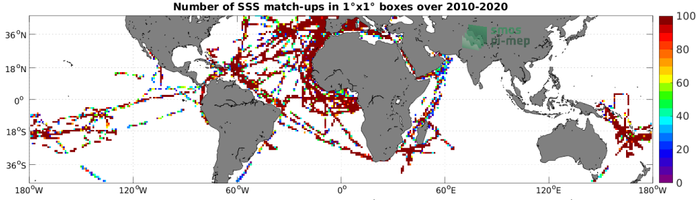
Figure 4: Number of SSS match-ups between TSG (GOSUD-Research-vessel) SSS and the SMOS SSS L2Q v331 - No FLAG (CMEMS-CATDS-CPDC) SSS product for the Mid-Low Latitudes 45N-45S Pi-MEP region over 1^\circ \times 1^\circ boxes and for the full satellite product period.
