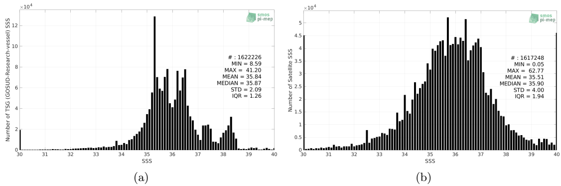
Figure 2: Histograms of SSS from TSG (GOSUD-Research-vessel) (a) and SMOS SSS L2Q v331 - No FLAG (CMEMS-CATDS-CPDC) (b) considering all match-up pairs per bins of 0.1 over the Mid-Low Latitudes 45N-45S Pi-MEP region and for the full satellite product period.
