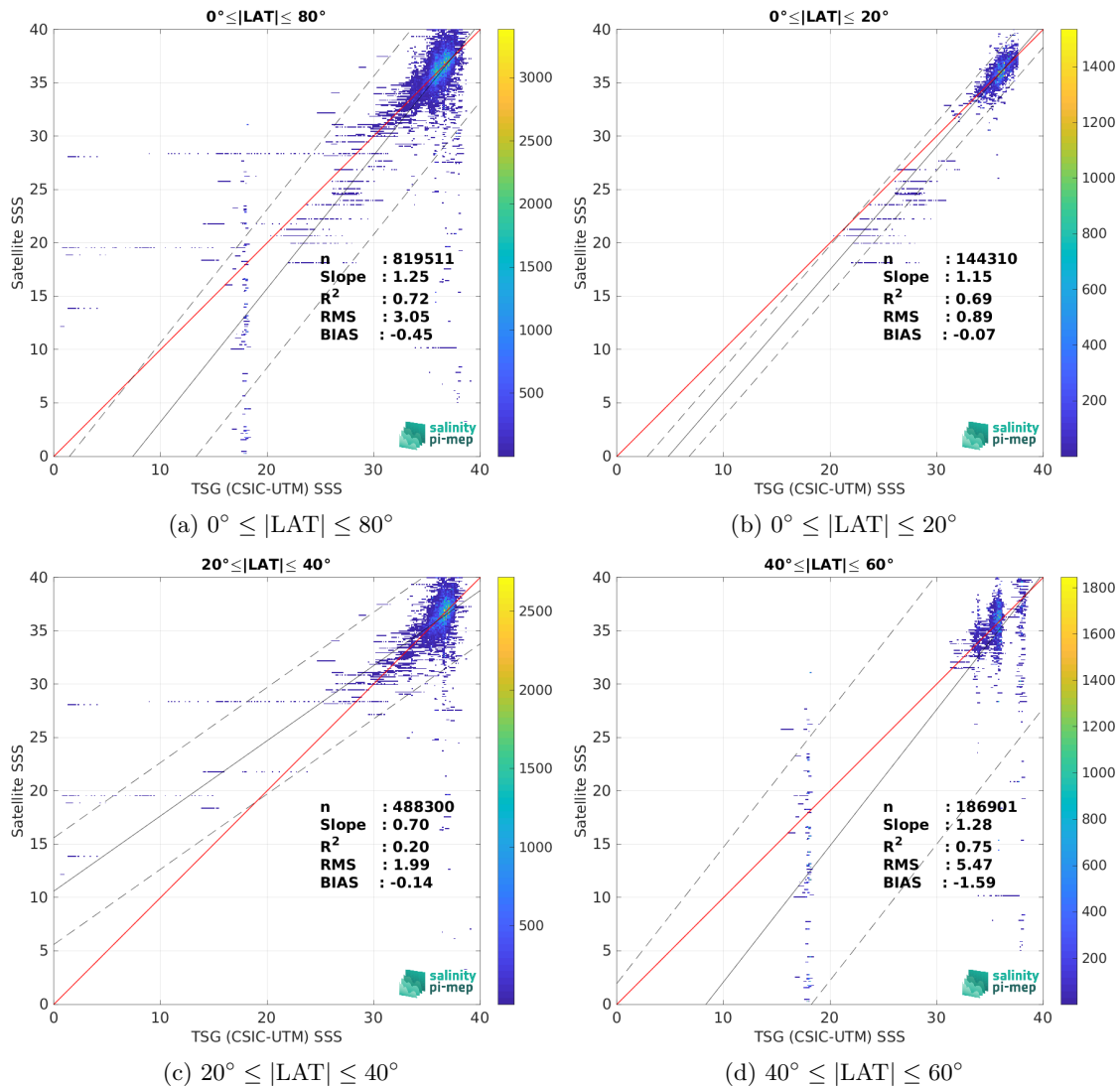
Figure 10: Contour maps of the concentration of SMOS SSS L2Q v331 - No FLAG (CMEMS-CATDS-CPDC) SSS (y-axis) versus TSG (CSIC-UTM) SSS (x-axis) at match-up pairs for different latitude bands. For each plot, the red line shows x=y . The black thin and dashed lines indicate a linear fit through the data cloud and the \pm 95\% confidence levels, respectively. The number match-up pairs n , the slope and R^2 coefficient of the linear fit, the root mean square (RMS) and the mean bias between satellite and in situ data are indicated for each latitude band in each plots.
