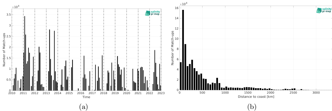
Figure 2: Number of match-ups between TSG (CSIC-UTM) and SMOS SSS L2Q v331 - No FLAG (CMEMS-CATDS-CPDC) SSS as a function of time (a) and as function of the distance to coast (b) over the Mid-Low Latitudes 45N-45S Pi-MEP region and for the full satellite product period.
