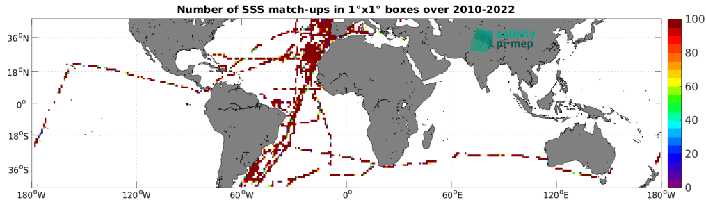
Figure 5: Number of SSS match-ups between TSG (CSIC-UTM) SSS and the SMOS SSS L2Q v331 - No FLAG (CMEMS-CATDS-CPDC) SSS product for the Mid-Low Latitudes 45N-45S Pi-MEP region over 1^\circ \times 1^\circ boxes and for the full satellite product period.
