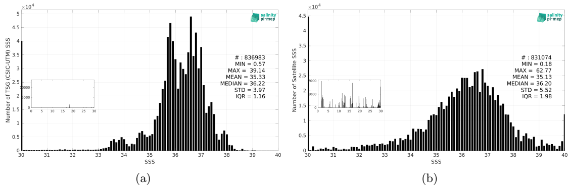
Figure 3: Histograms of SSS from TSG (CSIC-UTM) (a) and SMOS SSS L2Q v331 - No FLAG (CMEMS-CATDS-CPDC) (b) considering all match-up pairs per bins of 0.1 over the Mid-Low Latitudes 45N-45S Pi-MEP region and for the full satellite product period.
