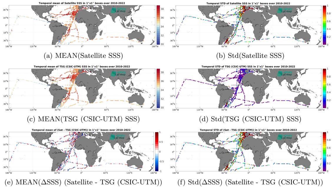
Figure 7: Temporal mean (left) and Std (right) of SSS from SMOS SSS L2Q v331 - No FLAG (CMEMS-CATDS-CPDC) (top), TSG (CSIC-UTM) (middle), and of \Delta SSS (Satellite - TSG (CSIC-UTM)). Only match-up pairs are used to generate these maps.
