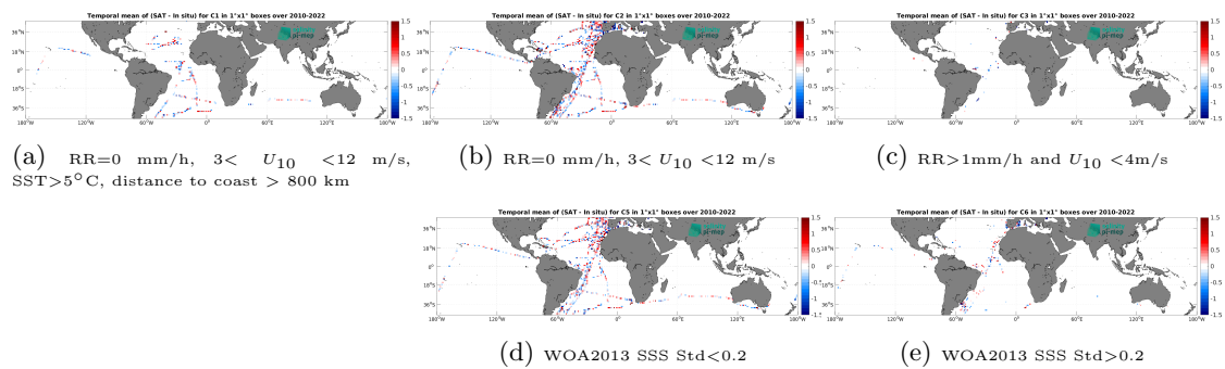
Figure 14: Temporal mean gridded over spatial boxes of size 1^\circ \times 1^\circ of \Delta SSS (SMOS SSS L2Q v331 - No FLAG (CMEMS-CATDS-CPDC) - TSG (CSIC-UTM)) for 5 different subdatasets corresponding to: RR=0 mm/h, 3 < U_{10} < 12 m/s, SST > 5°C, distance to coast > 800 km (a), RR=0 mm/h, 3 < U_{10} < 12 m/s (b), RR > 1mm/h and U_{10} < 4 m/s (c), WOA2013 SSS Std < 0.2 (d), WOA2013 SSS Std > 0.2 (e).
