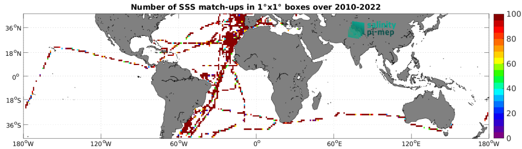
Figure 4: Number of SSS match-ups between TSG (CSIC-UTM) SSS and the SMOS SSS L2Q v331 - No FLAG (CMEMS-CATDS-CPDC) SSS product for the Mid-Low Latitudes 45N-45S Pi-MEP region over 1^\circ \times 1^\circ boxes and for the full satellite product period.
