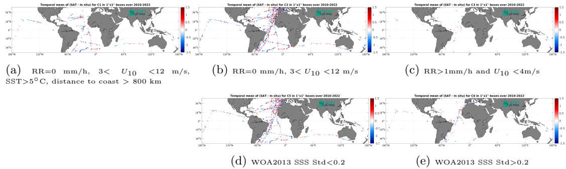
Figure 12: Temporal mean gridded over spatial boxes of size 1^\circ \times 1^\circ of \Delta SSS (SMOS SSS L2Q v331 - No FLAG (CMEMS-CATDS-CPDC) - TSG (CSIC-UTM)) for 5 different subdatasets corresponding to:RR=0 mm/h, 3 < U_{10} < 12 m/s, SST >5^\circ C, distance to coast > 800 km (a), RR=0 mm/h, 3 < U_{10} < 12 m/s (b), RR >1 mm/h and U_{10} < 4 m/s (c), WOA2013 SSS Std <0.2 (d), WOA2013 SSS Std >0.2 (e).
