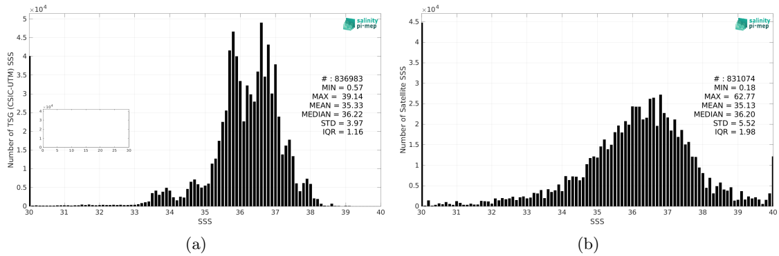
Figure 2: Histograms of SSS from TSG (CSIC-UTM) (a) and SMOS SSS L2Q v331 - No FLAG (CMEMS-CATDS-CPDC) (b) considering all match-up pairs per bins of 0.1 over the Mid-Low Latitudes 45N-45S Pi-MEP region and for the full satellite product period.
