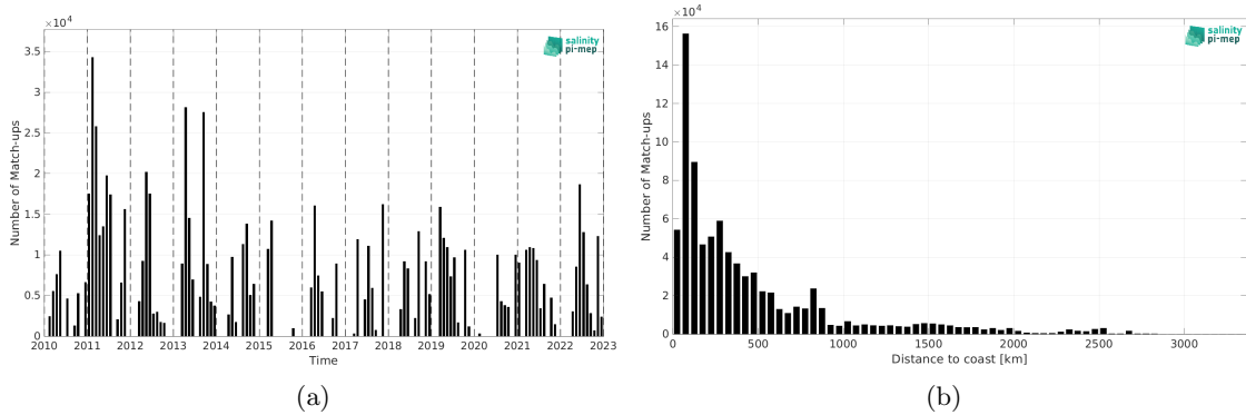
Figure 1: Number of match-ups between TSG (CSIC-UTM) and SMOS SSS L2Q v331 - No FLAG (CMEMS-CATDS-CPDC) SSS as a function of time (a) and as function of the distance to coast (b) over the Mid-Low Latitudes 45N-45S Pi-MEP region and for the full satellite product period.
