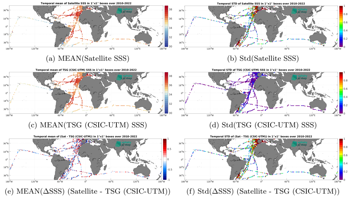
Figure 6: Temporal mean (left) and Std (right) of SSS from SMOS SSS L2Q v331 - No FLAG (CMEMS-CATDS-CPDC) (top), TSG (CSIC-UTM) (middle), and of \Delta SSS (Satellite - TSG (CSIC-UTM)). Only match-up pairs are used to generate these maps.
