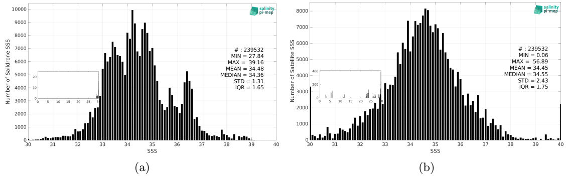
Figure 3: Histograms of SSS from Saildrone (a) and SMOS SSS L2Q v331 - No FLAG (CMEMS-CATDS-CPDC) (b) considering all match-up pairs per bins of 0.1 over the Mid-Low Latitudes 45N-45S Pi-MEP region and for the full satellite product period.
