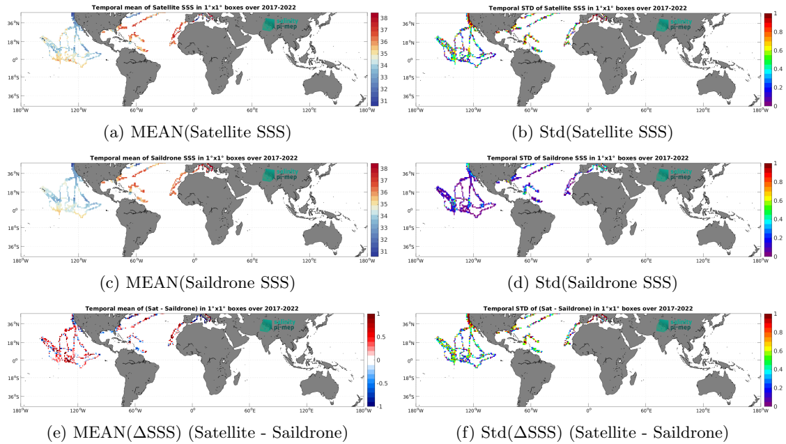
Figure 7: Temporal mean (left) and Std (right) of SSS from SMOS SSS L2Q v331 - No FLAG (CMEMS-CATDS-CPDC) (top), Saildrone (middle), and of \Delta SSS (Satellite - Saildrone). Only match-up pairs are used to generate these maps.
