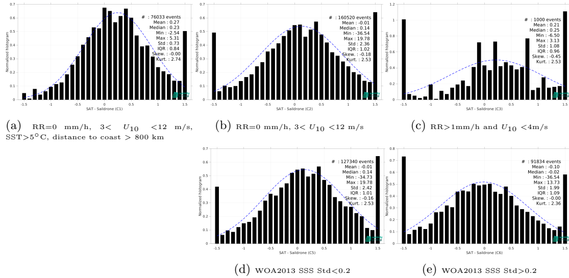
Figure 15: Normalized histogram of \Delta SSS (SMOS SSS L2Q v331 - No FLAG (CMEMS-CATDS-CPDC) - Saildrone) for 5 different subdatasets corresponding to: RR=0 mm/h, 3 < U_{10} < 12 m/s, SST>5°C, distance to coast > 800 km (a), RR=0 mm/h, 3 < U_{10} < 12 m/s (b), RR>1mm/h and U_{10} < 4 m/s (c), WOA2013 SSS Std<0.2 (d), WOA2013 SSS Std>0.2 (e).
