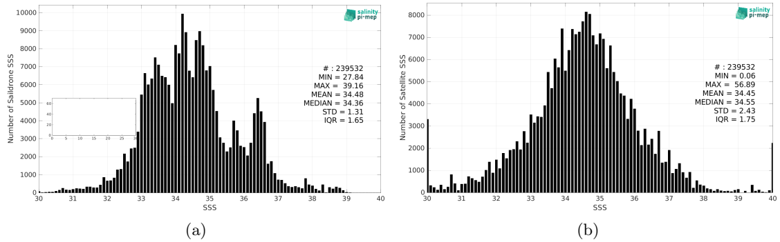
Figure 2: Histograms of SSS from Saildrone (a) and SMOS SSS L2Q v331 - No FLAG (CMEMS-CATDS-CPDC) (b) considering all match-up pairs per bins of 0.1 over the Mid-Low Latitudes 45N-45S Pi-MEP region and for the full satellite product period.
