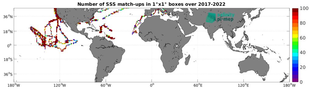
Figure 4: Number of SSS match-ups between Saildrone SSS and the SMOS SSS L2Q v331 - No FLAG (CMEMS-CATDS-CPDC) SSS product for the Mid-Low Latitudes 45N-45S Pi-MEP region over 1^{\circ} \times 1^{\circ} boxes and for the full satellite product period.
