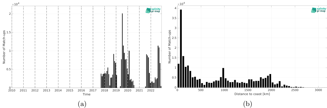
Figure 1: Number of match-ups between Saildrone and SMOS SSS L2Q v331 - No FLAG (CMEMS-CATDS-CPDC) SSS as a function of time (a) and as function of the distance to coast (b) over the Mid-Low Latitudes 45N-45S Pi-MEP region and for the full satellite product period.
