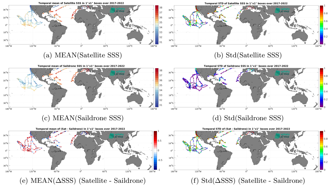
Figure 6: Temporal mean (left) and Std (right) of SSS from SMOS SSS L2Q v331 - No FLAG (CMEMS-CATDS-CPDC) (top), Saildrone (middle), and of \Delta SSS (Satellite - Saildrone). Only match-up pairs are used to generate these maps.
