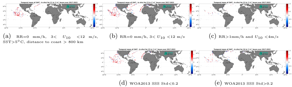
Figure 12: Temporal mean gridded over spatial boxes of size 1^\circ \times 1^\circ of \Delta SSS (SMOS SSS L2Q v331 - No FLAG (CMEMS-CATDS-CPDC) - Saildrone) for 5 different subdatasets corresponding to:RR=0 mm/h, 3 < U_{10} < 12 m/s, SST >5^\circ C, distance to coast > 800 km (a), RR=0 mm/h, 3 < U_{10} < 12 m/s (b), RR >1 mm/h and U_{10} < 4 m/s (c), WOA2013 SSS Std <0.2 (d), WOA2013 SSS Std >0.2 (e).
