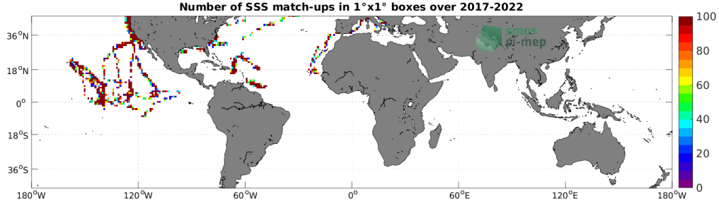
Figure 4: Number of SSS match-ups between Saildrone SSS and the SMOS SSS L2Q v331 - No FLAG (CMEMS-CATDS-CPDC) SSS product for the Mid-Low Latitudes 45N-45S Pi-MEP region over 1^\circ \times 1^\circ boxes and for the full satellite product period.
