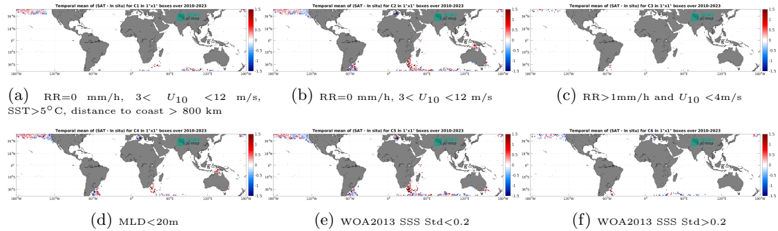
Figure 14: Temporal mean gridded over spatial boxes of size 1^\circ \times 1^\circ of \Delta SSS (SMOS SSS L2Q v331 - No FLAG (CMEMS-CATDS-CPDC) - Marine mammals) for 6 different subdatasets corresponding to:RR=0 mm/h, 3 < U_{10} < 12 m/s, SST >5^\circ\text{C} , distance to coast > 800 km (a), RR=0 mm/h, 3 < U_{10} < 12 m/s (b), RR >1 mm/h and U_{10} < 4 m/s (c),MLD <20 m (d),WOA2013 SSS Std <0.2 (e),WOA2013 SSS Std >0.2 (f).
