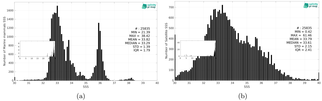
Figure 3: Histograms of SSS from Marine mammals (a) and SMOS SSS L2Q v331 - No FLAG (CMEMS-CATDS-CPDC) (b) considering all match-up pairs per bins of 0.1 over the Mid-Low Latitudes 45N-45S Pi-MEP region and for the full satellite product period.
