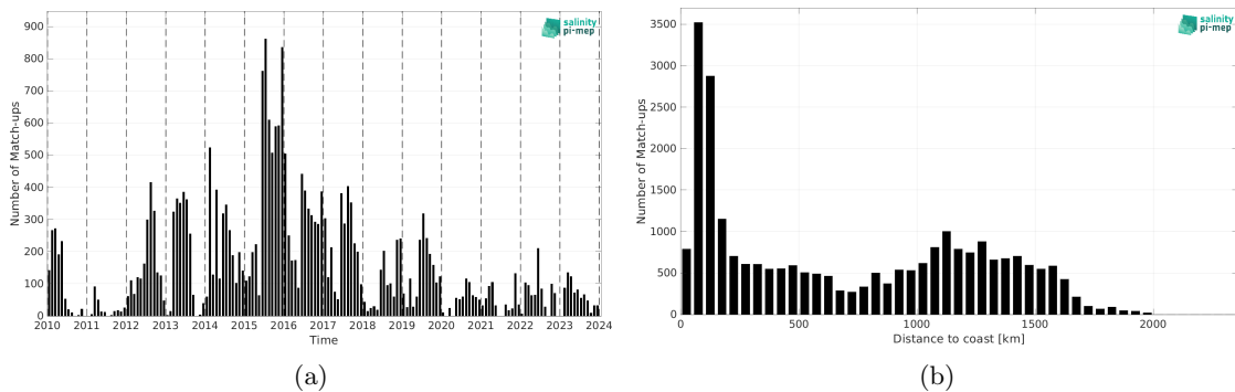
Figure 2: Number of match-ups between Marine mammals and SMOS SSS L2Q v331 - No FLAG (CMEMS-CATDS-CPDC) SSS as a function of time (a) and as function of the distance to coast (b) over the Mid-Low Latitudes 45N-45S Pi-MEP region and for the full satellite product period.
