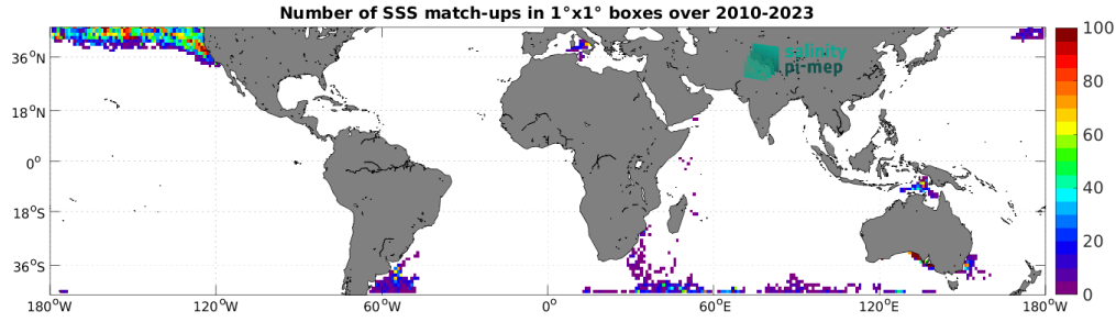
Figure 5: Number of SSS match-ups between Marine mammals SSS and the SMOS SSS L2Q v331 - No FLAG (CMEMS-CATDS-CPDC) SSS product for the Mid-Low Latitudes 45N-45S Pi-MEP region over 1^{\circ} \times 1^{\circ} boxes and for the full satellite product period.
