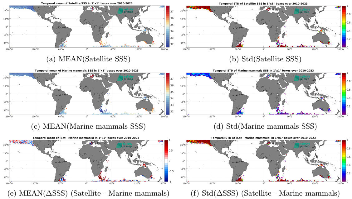
Figure 7: Temporal mean (left) and Std (right) of SSS from SMOS SSS L2Q v331 - No FLAG (CMEMS-CATDS-CPDC) (top), Marine mammals (middle), and of \Delta SSS (Satellite - Marine mammals). Only match-up pairs are used to generate these maps.
