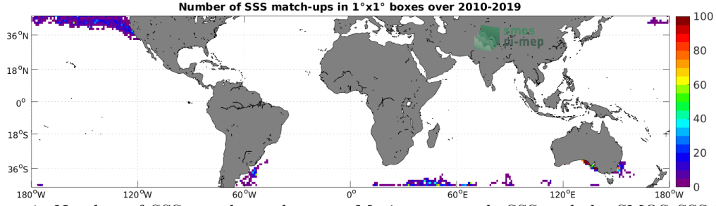
Figure 4: Number of SSS match-ups between Marine mammals SSS and the SMOS SSS L2Q v331 - No FLAG (CMEMS-CATDS-CPDC) SSS product for the Mid-Low Latitudes 45N-45S Pi-MEP region over 1^\circ \times 1^\circ boxes and for the full satellite product period.
