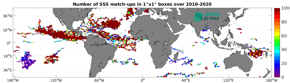
Figure 4: Number of SSS match-ups between Surface drifters SSS and the SMOS SSS L2Q v331 - No FLAG (CMEMS-CATDS-CPDC) SSS product for the Mid-Low Latitudes 45N-45S Pi-MEP region over 1^\circ \times 1^\circ boxes and for the full satellite product period.
