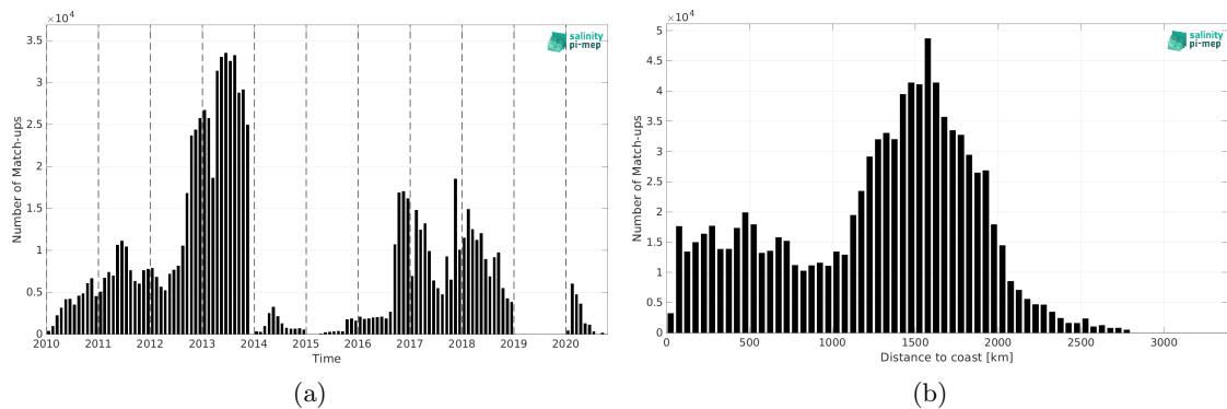
Figure 2: Number of match-ups between Surface drifters and SMOS SSS L2Q v331 - No FLAG (CMEMS-CATDS-CPDC) SSS as a function of time (a) and as function of the distance to coast (b) over the Mid-Low Latitudes 45N-45S Pi-MEP region and for the full satellite product period.
