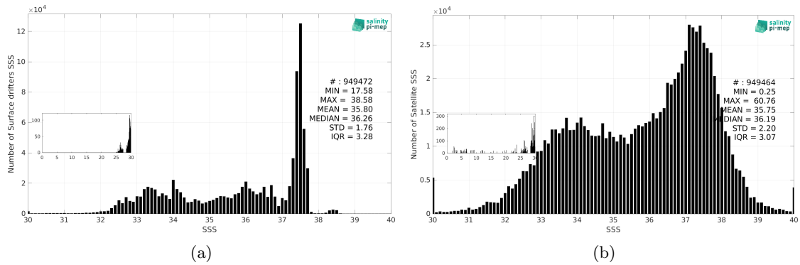
Figure 3: Histograms of SSS from Surface drifters (a) and SMOS SSS L2Q v331 - No FLAG (CMEMS-CATDS-CPDC) (b) considering all match-up pairs per bins of 0.1 over the Mid-Low Latitudes 45N-45S Pi-MEP region and for the full satellite product period.
