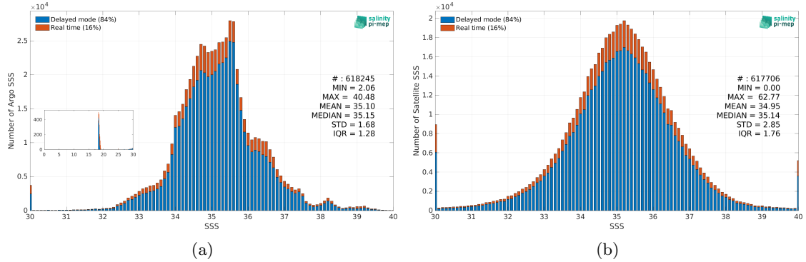
Figure 2: Histograms of SSS from Argo (a) and SMOS SSS L2Q v331 - No FLAG (CMEMS-CATDS-CPDC) (b) considering all match-up pairs per bins of 0.1 over the Mid-Low Latitudes 45N-45S Pi-MEP region and for the full satellite product period.
