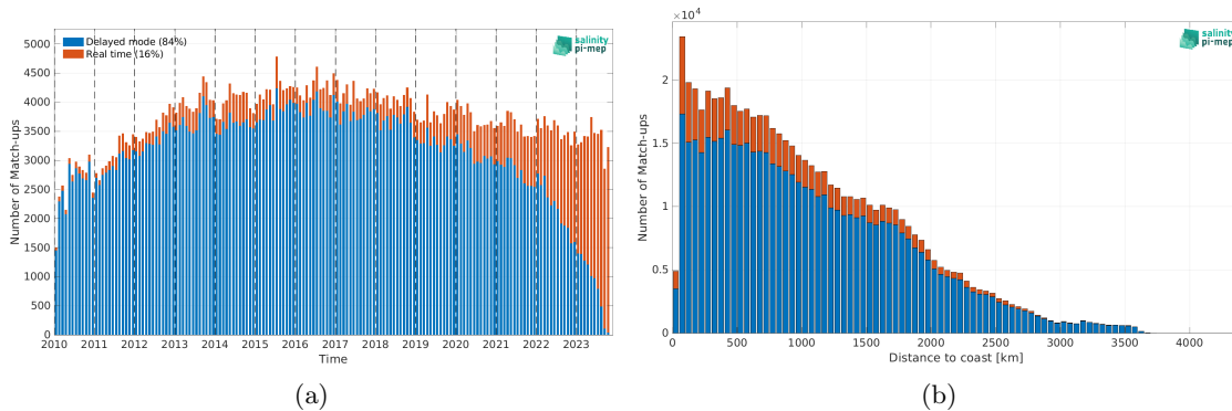
Figure 1: Number of match-ups between Argo and SMOS SSS L2Q v331 - No FLAG (CMEMS-CATDS-CPDC) SSS as a function of time (a) and as function of the distance to coast (b) over the Mid-Low Latitudes 45N-45S Pi-MEP region and for the full satellite product period.
