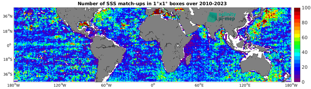
Figure 4: Number of SSS match-ups between Argo SSS and the SMOS SSS L2Q v331 - No FLAG (CMEMS-CATDS-CPDC) SSS product for the Mid-Low Latitudes 45N-45S Pi-MEP region over 1^\circ \times 1^\circ boxes and for the full satellite product period.
