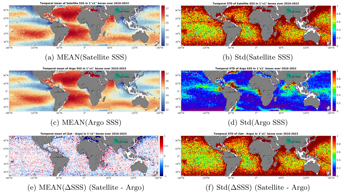
Figure 6: Temporal mean (left) and Std (right) of SSS from SMOS SSS L2Q v331 - No FLAG (CMEMS-CATDS-CPDC) (top), Argo (middle), and of \Delta SSS (Satellite - Argo). Only match-up pairs are used to generate these maps.
