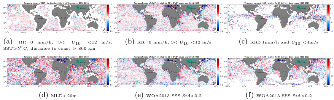
Figure 12: Temporal mean gridded over spatial boxes of size 1^\circ \times 1^\circ of \Delta SSS (SMOS SSS L2Q v331 - No FLAG (CMEMS-CATDS-CPDC) - Argo) for 6 different subdatasets corresponding to:RR=0 mm/h, 3 < U_{10} < 12 m/s, SST >5^\circ C, distance to coast > 800 km (a), RR=0 mm/h, 3 < U_{10} < 12 m/s (b), RR >1 mm/h and U_{10} < 4 m/s (c),MLD <20 m (d),WOA2013 SSS Std <0.2 (e),WOA2013 SSS Std >0.2 (f).
