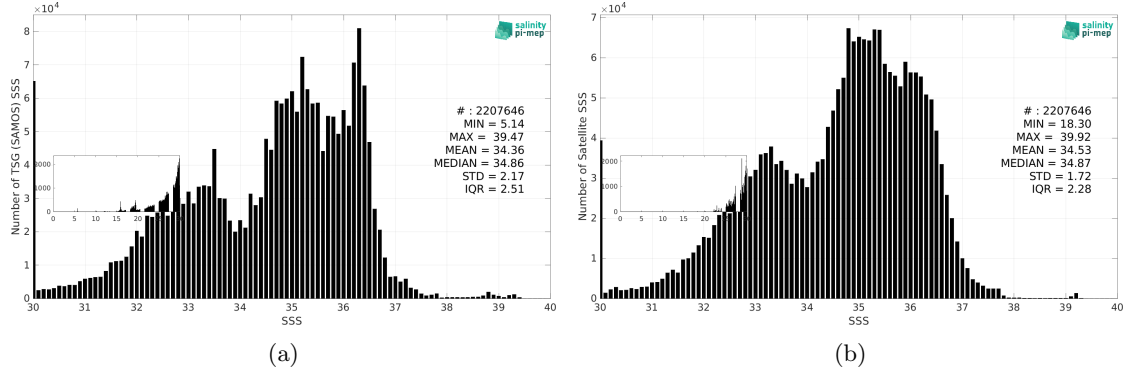
Figure 3: Histograms of SSS from TSG (SAMOS) (a) and SMOS SSS L3 v9 - 9 Days (CATDS-CEC-LOCEAN) (b) considering all match-up pairs per bins of 0.1 over the Mid-Low Latitudes 45N-45S Pi-MEP region and for the full satellite product period.
