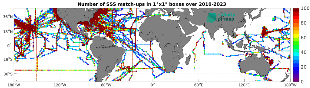
Figure 5: Number of SSS match-ups between TSG (SAMOS) SSS and the SMOS SSS L3 v9 - 9 Days (CATDS-CEC-LOCEAN) SSS product for the Mid-Low Latitudes 45N-45S Pi-MEP region over 1^\circ \times 1^\circ boxes and for the full satellite product period.
