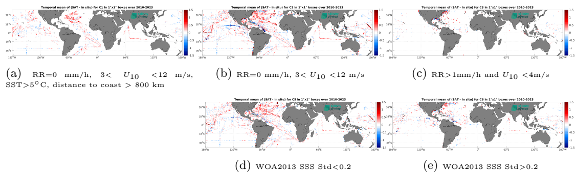
Figure 14: Temporal mean gridded over spatial boxes of size 1^\circ \times 1^\circ of \Delta SSS (SMOS SSS L3 v9 - 9 Days (CATDS-CEC-LOCEAN) - TSG (SAMOS)) for 5 different subdatasets corresponding to: RR=0 mm/h, 3 < U_{10} < 12 m/s, SST > 5°C, distance to coast > 800 km (a), RR=0 mm/h, 3 < U_{10} < 12 m/s (b), RR > 1mm/h and U_{10} < 4 m/s (c), WOA2013 SSS Std < 0.2 (d), WOA2013 SSS Std > 0.2 (e).
