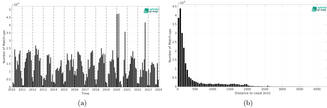
Figure 2: Number of match-ups between TSG (SAMOS) and SMOS SSS L3 v9 - 9 Days (CATDS-CEC-LOCEAN) SSS as a function of time (a) and as function of the distance to coast (b) over the Mid-Low Latitudes 45N-45S Pi-MEP region and for the full satellite product period.
