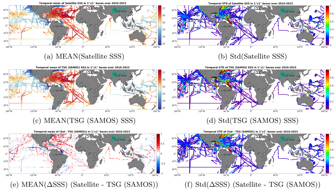
Figure 7: Temporal mean (left) and Std (right) of SSS from SMOS SSS L3 v9 - 9 Days (CATDS-CEC-LOCEAN) (top), TSG (SAMOS) (middle), and of \Delta SSS (Satellite - TSG (SAMOS)). Only match-up pairs are used to generate these maps.
