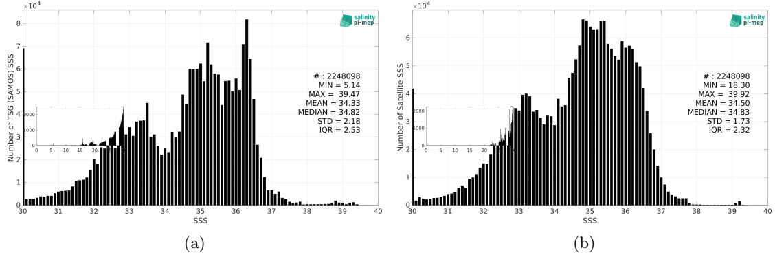
Figure 2: Histograms of SSS from TSG (SAMOS) (a) and SMOS SSS L3 v9 - 9 Days (CATDS-CEC-LOCEAN) (b) considering all match-up pairs per bins of 0.1 over the Mid-Low Latitudes 45N-45S Pi-MEP region and for the full satellite product period.
