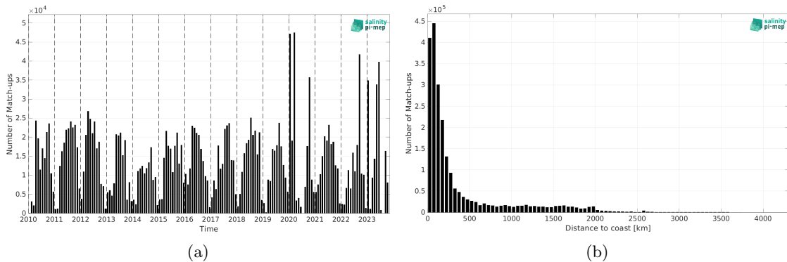
Figure 1: Number of match-ups between TSG (SAMOS) and SMOS SSS L3 v9 - 9 Days (CATDS-CEC-LOCEAN) SSS as a function of time (a) and as function of the distance to coast (b) over the Mid-Low Latitudes 45N-45S Pi-MEP region and for the full satellite product period.
