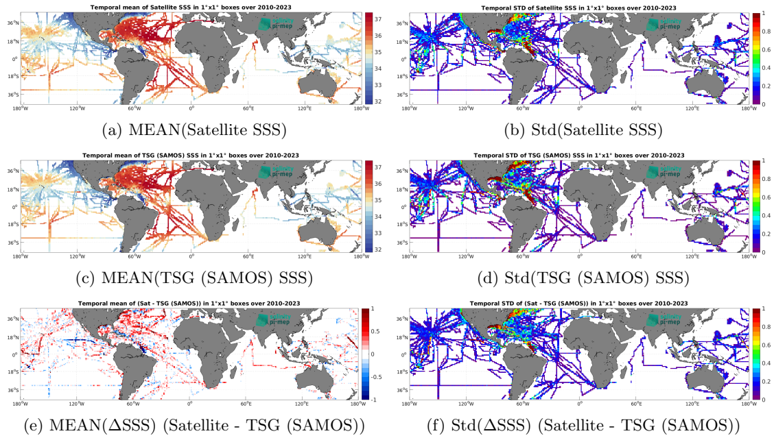
Figure 6: Temporal mean (left) and Std (right) of SSS from SMOS SSS L3 v9 - 9 Days (CATDS-CEC-LOCEAN) (top), TSG (SAMOS) (middle), and of \Delta SSS (Satellite - TSG (SAMOS)). Only match-up pairs are used to generate these maps.
