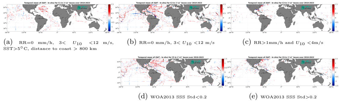
Figure 12: Temporal mean gridded over spatial boxes of size 1^\circ \times 1^\circ of \Delta SSS (SMOS SSS L3 v9 - 9 Days (CATDS-CEC-LOCEAN) - TSG (SAMOS)) for 5 different subdatasets corresponding to:RR=0 mm/h, 3 < U_{10} < 12 m/s, SST >5^\circ\text{C} , distance to coast > 800 km (a), RR=0 mm/h, 3 < U_{10} < 12 m/s (b), RR >1 mm/h and U_{10} < 4 m/s (c), WOA2013 SSS Std <0.2 (d), WOA2013 SSS Std >0.2 (e).
