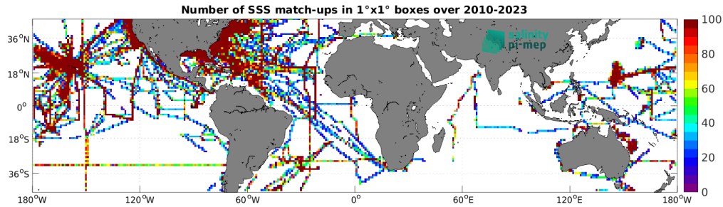
Figure 4: Number of SSS match-ups between TSG (SAMOS) SSS and the SMOS SSS L3 v9 - 9 Days (CATDS-CEC-LOCEAN) SSS product for the Mid-Low Latitudes 45N-45S Pi-MEP region over 1^\circ \times 1^\circ boxes and for the full satellite product period.
